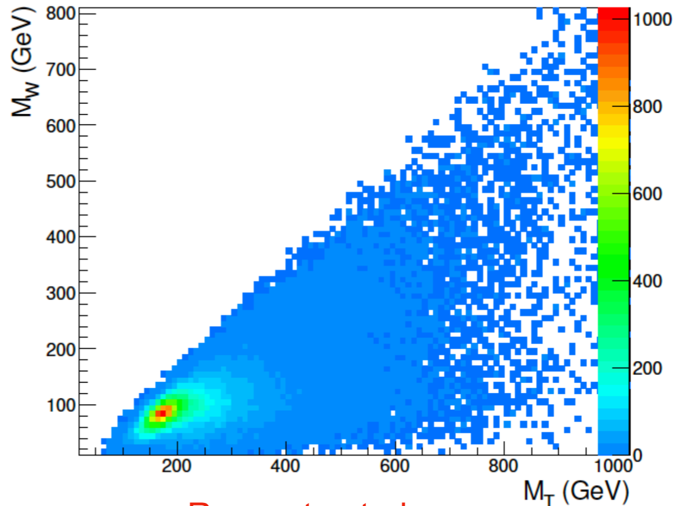
Reconstructed masses of both top quark and W boson
