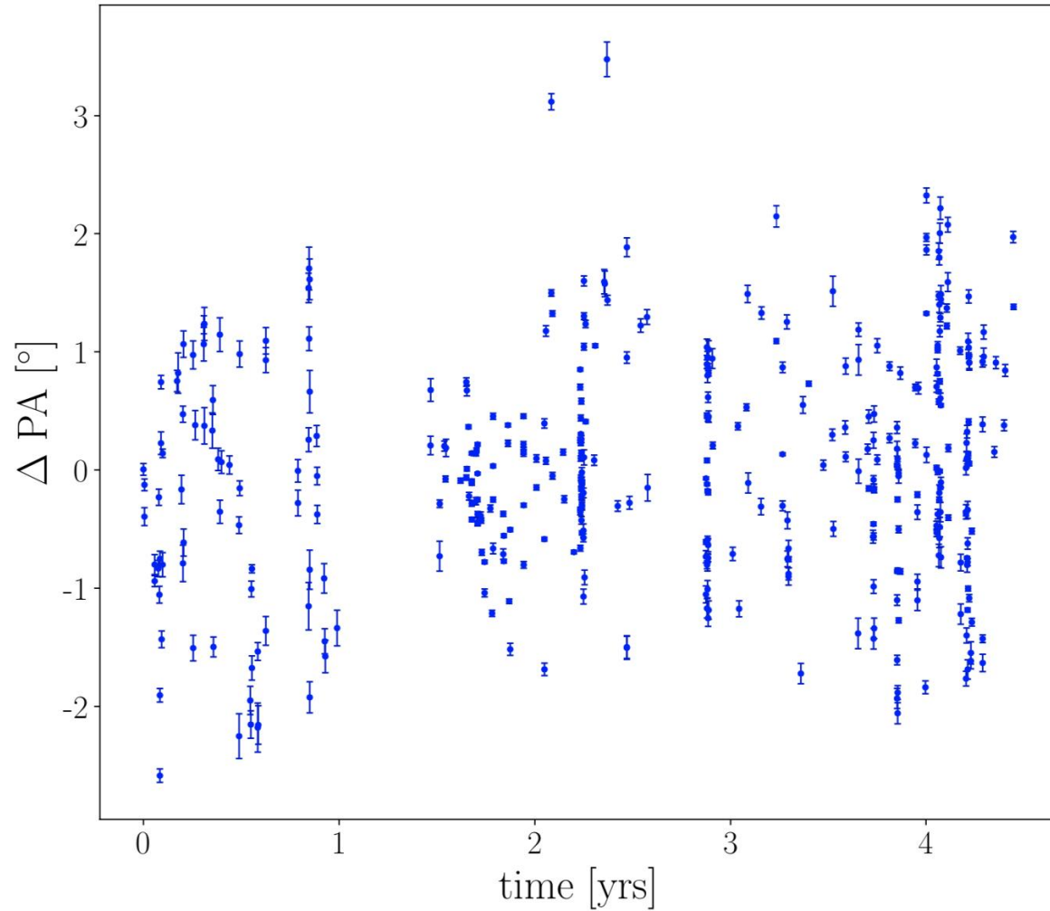
Real time series (with systematic corrections)
