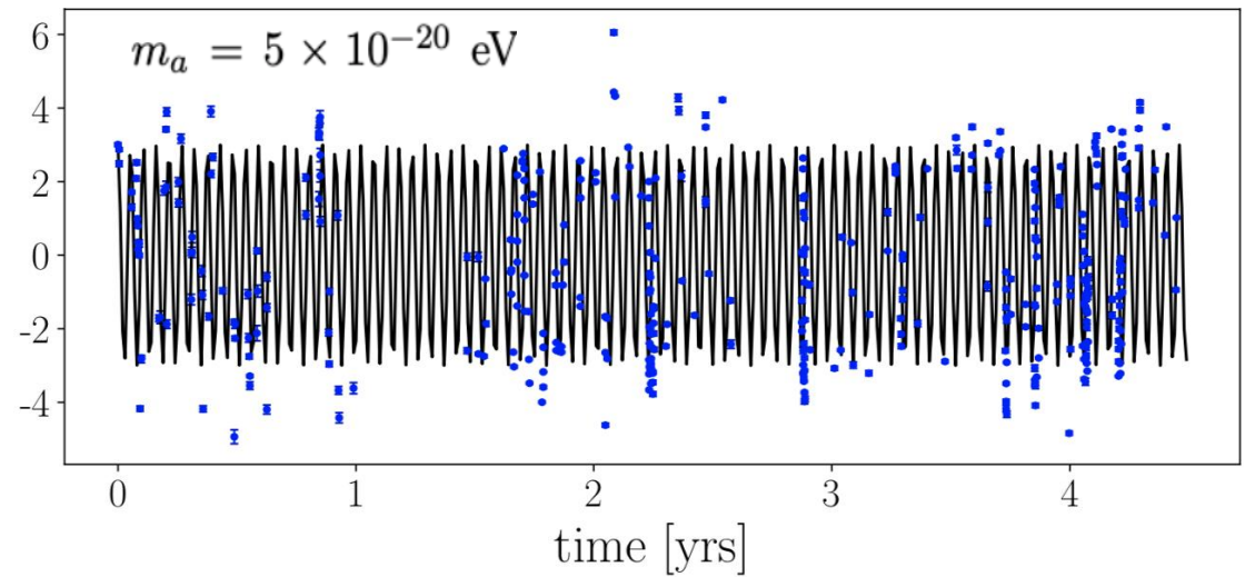
Expected time series with ALP effect
