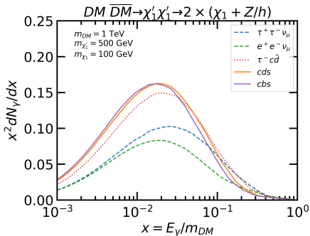
Figure 2: Left: Effective DM annihilation through a neutralino cascade. “RPV” indicates the three fermion final state from RPV \chi_1 decay, which differs based on the dominant RPV coupling. Right: The resulting spectra for specific examples of non-zero RPV couplings.
