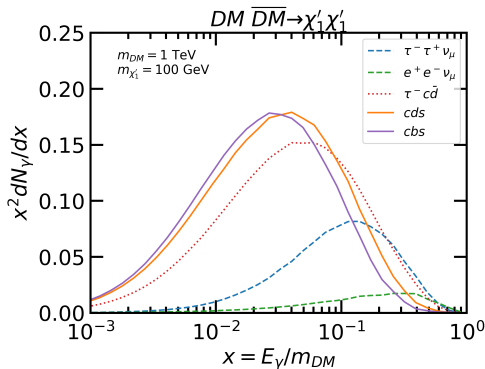
Figure 3: The photon spectra for direct \psi annihilation to \chi'_1 , shown for multiple potential RPV mediated \chi'_1 decays.
