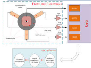
Figure 1. the diagram of the coincidence counting system
