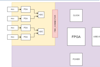
Figure 2. the diagram of self-designed digitalizer
