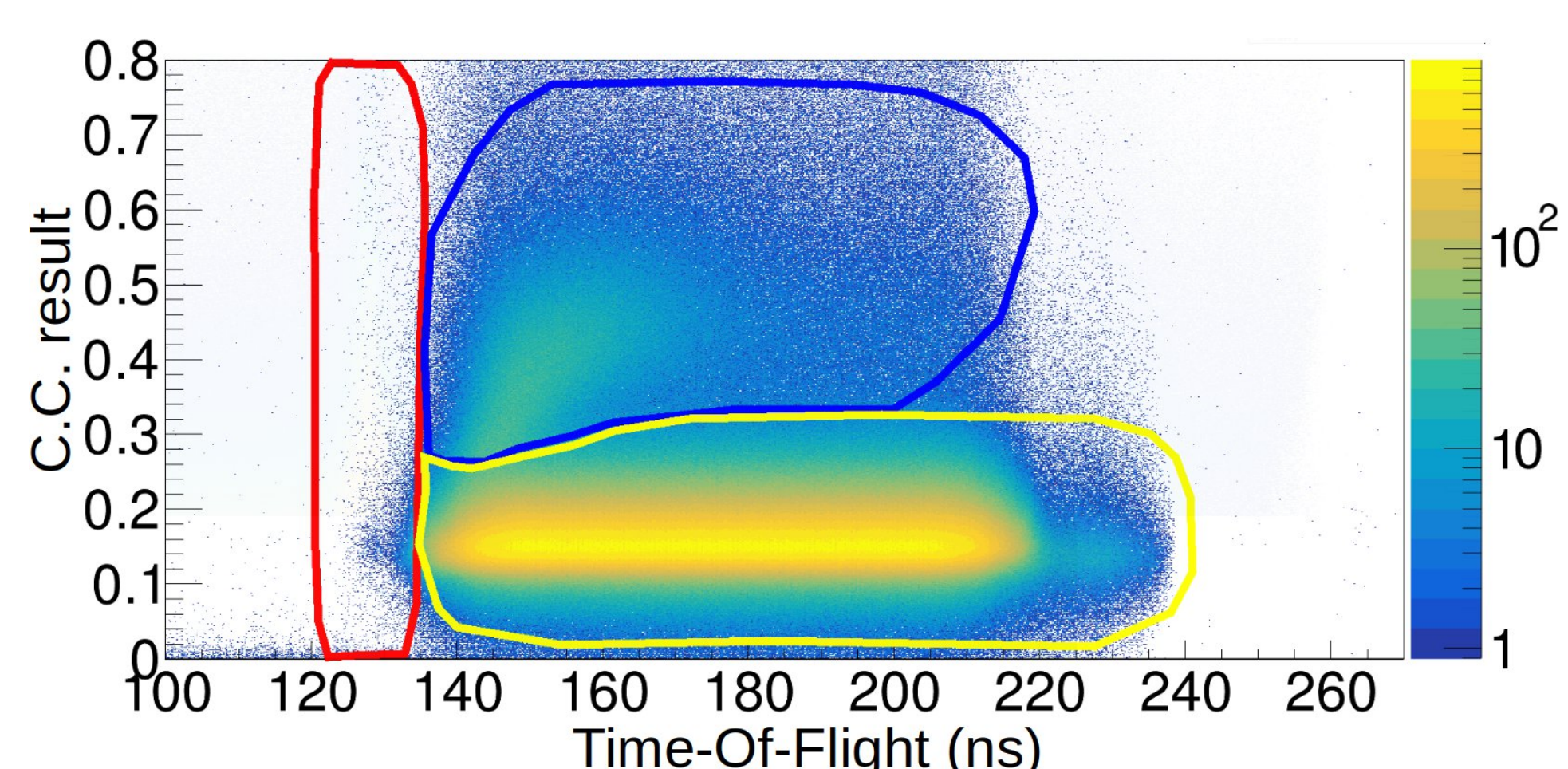
Figure 2. Event distribution using TOF trigger mode.
