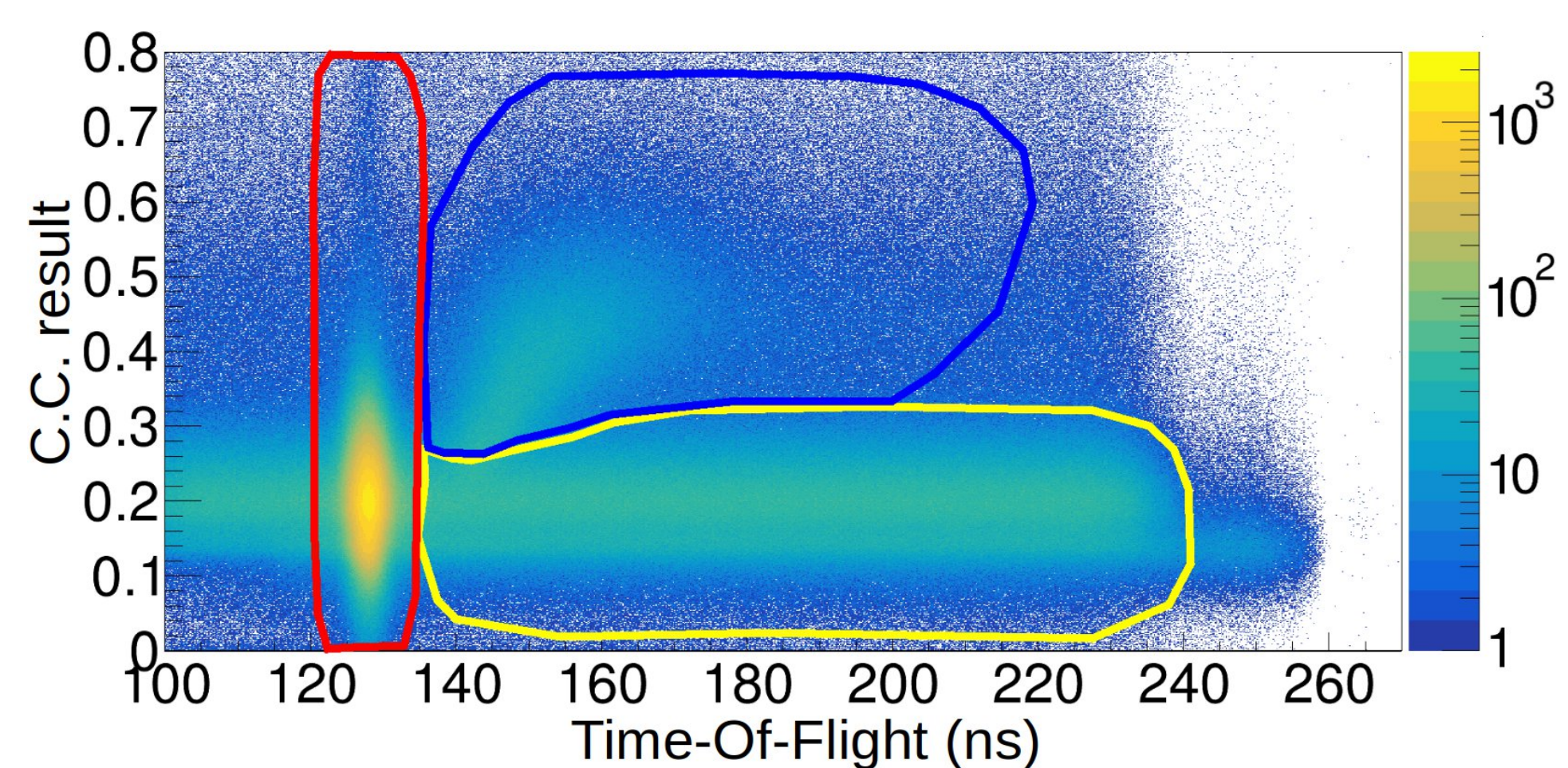
Figure 1. Event distribution using C.C. trigger mode.
