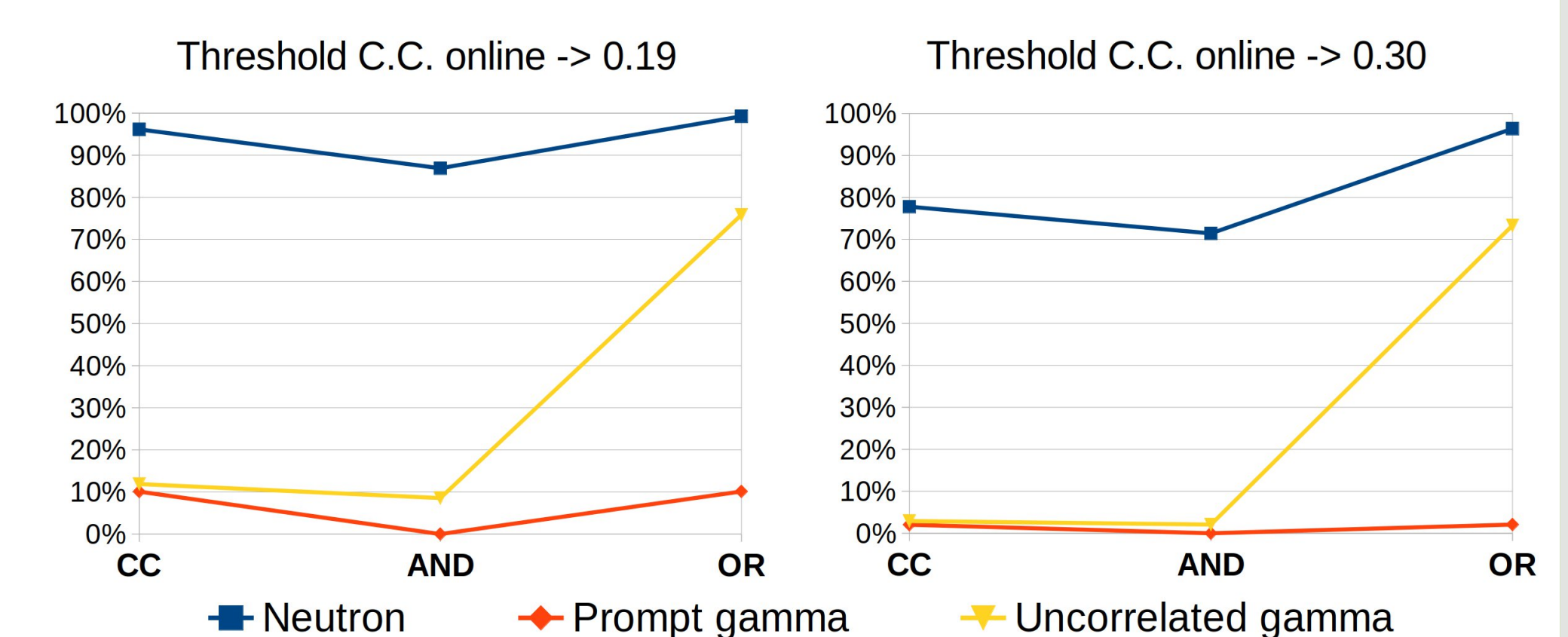
Figure 7. Percentage of events acquired compared to acquisition without trigger condition using different C.C. thresholds (0.19 and 0.30).
