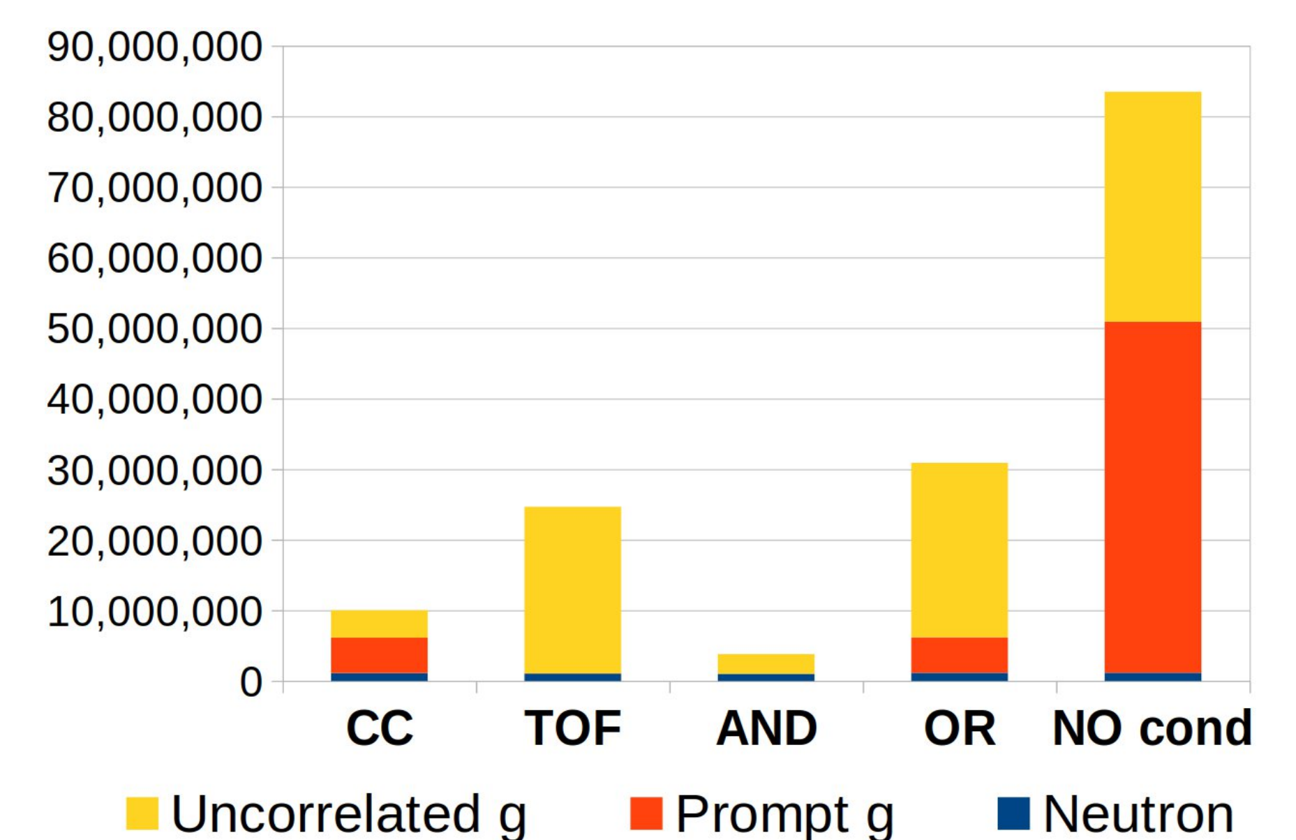
Figure 5. Number of events acquired with each trigger mode and for each type of particle.
