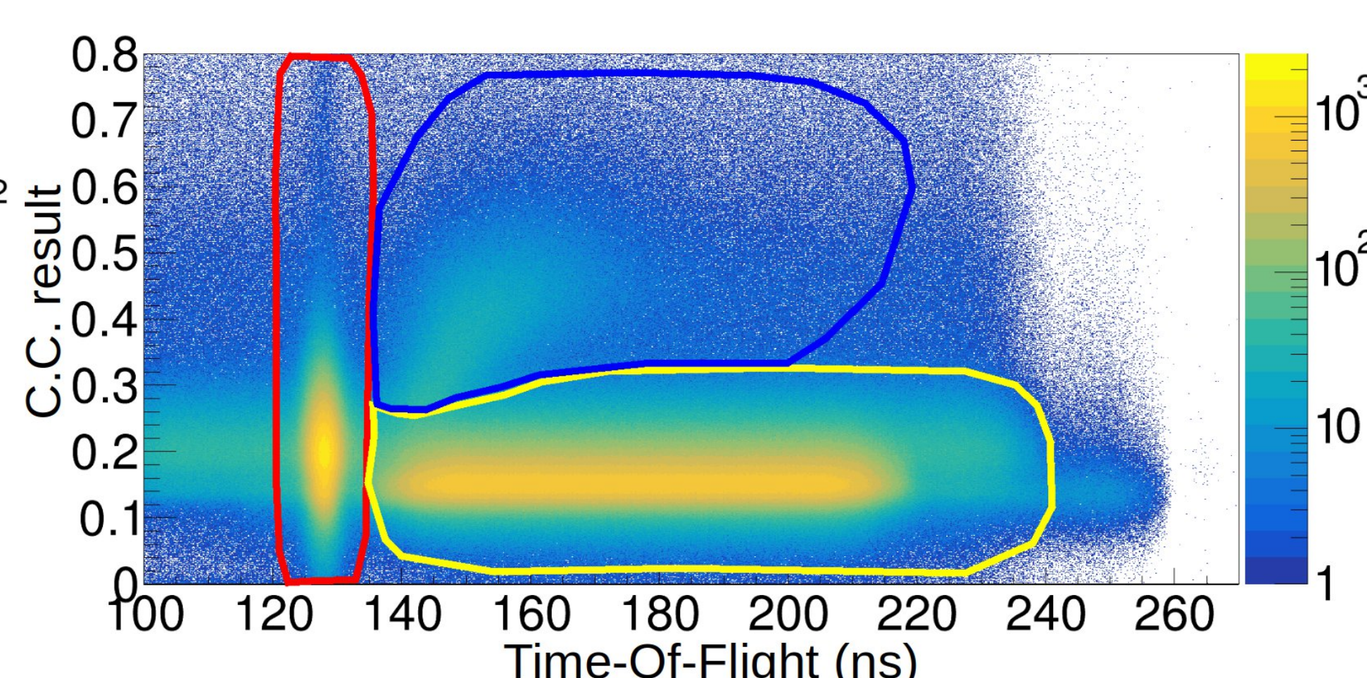
Figure 4. Event distribution using OR trigger mode.
