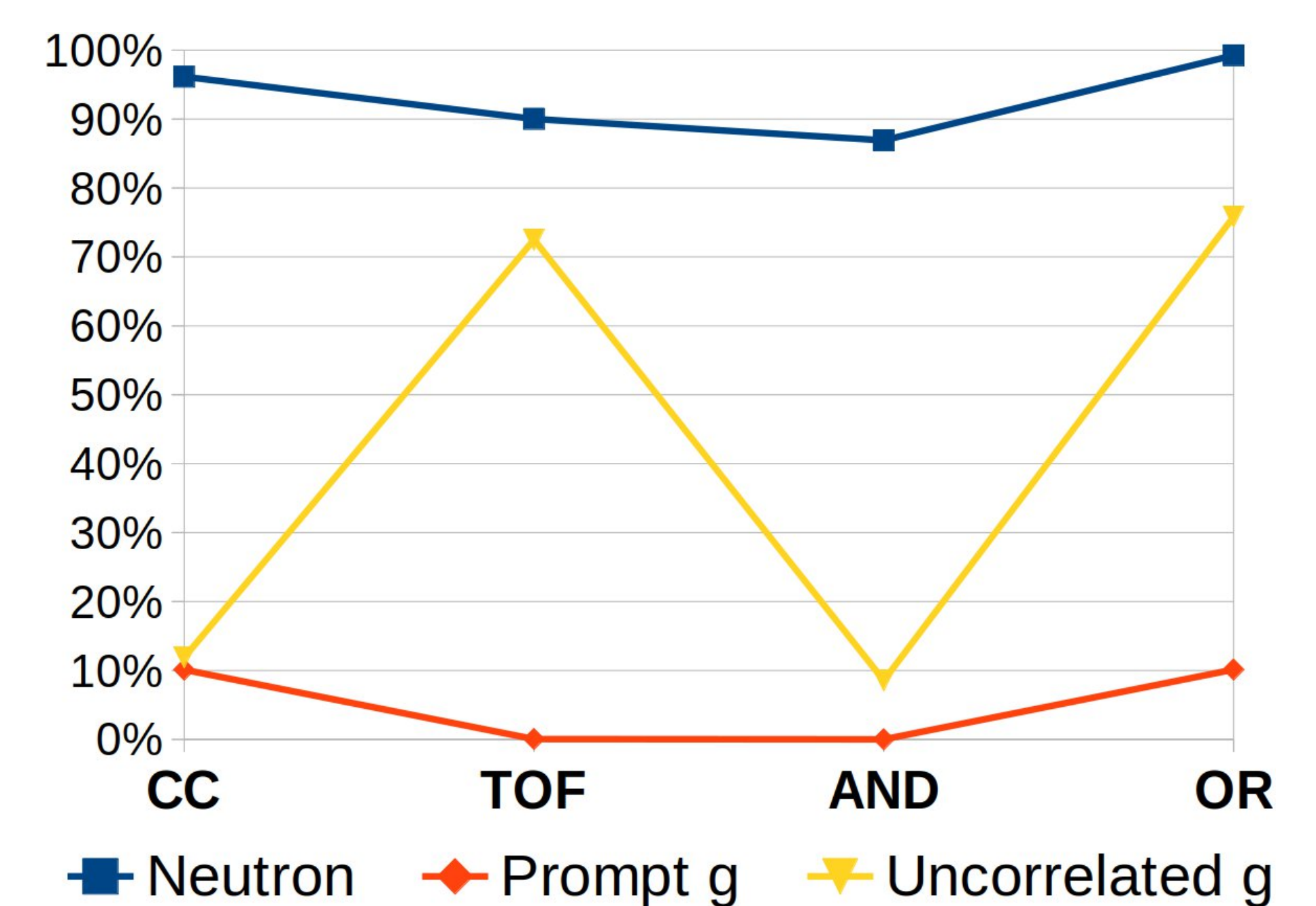
Figure 6. Percentage of events acquired by type of particle and by trigger mode compared to no trigger condition.
