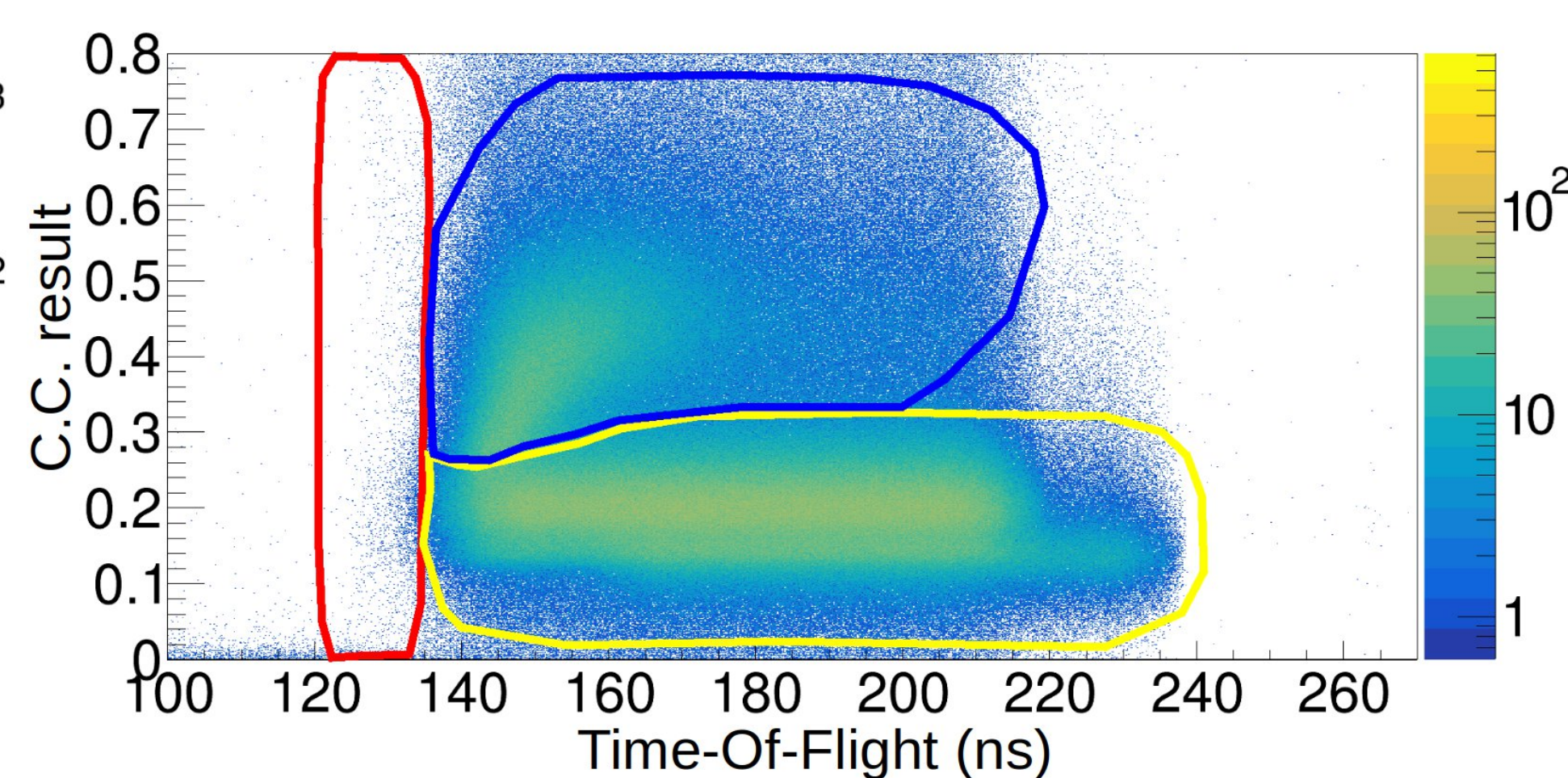
Figure 3. Event distribution using AND trigger mode.
