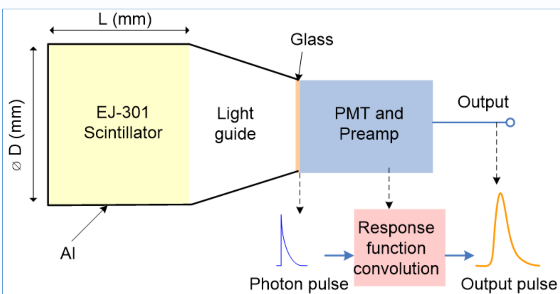
Fig. 1. Modeling the EJ-301 detector.
