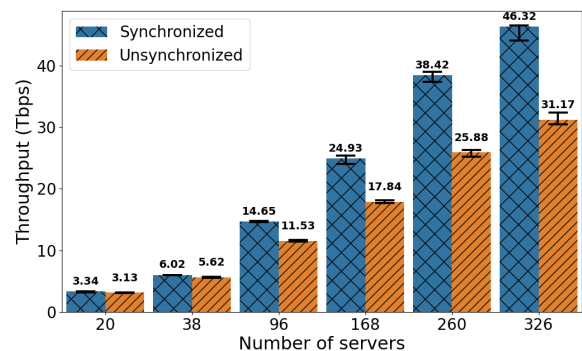
Fig. 6: Scalability of the synchronized and non-synchronized all-to-all applications. The error bars represent the minimum, mean and maximum values.
