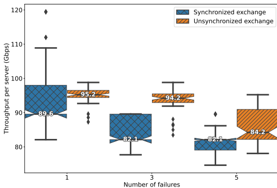
Fig. 7: Synchronized and non-synchronized all-to-all exchange throughput per server as a function of the number of failures. Failure scenarios are randomly generated 10 times for each number of failures. The number of simultaneous failures in the Event Builder network is 1, 3 or 5. The boxplots represent the minimum, 25th percentile, median, 75th percentile, and maximum values. Outliers are also depicted.
