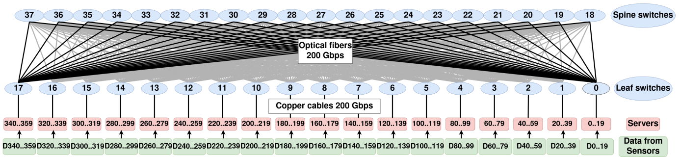
Fig. 1: The Event Builder Network of the LHCb experiment.
