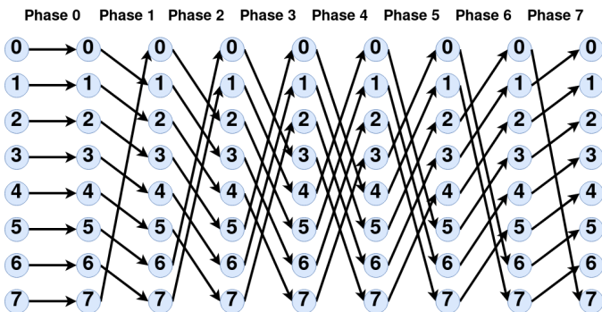
Fig. 2: The Linear-shift scheduling with 8 servers.
