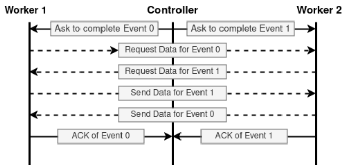
Fig. 5: Description of the MPI all-to-all application without synchronization.
