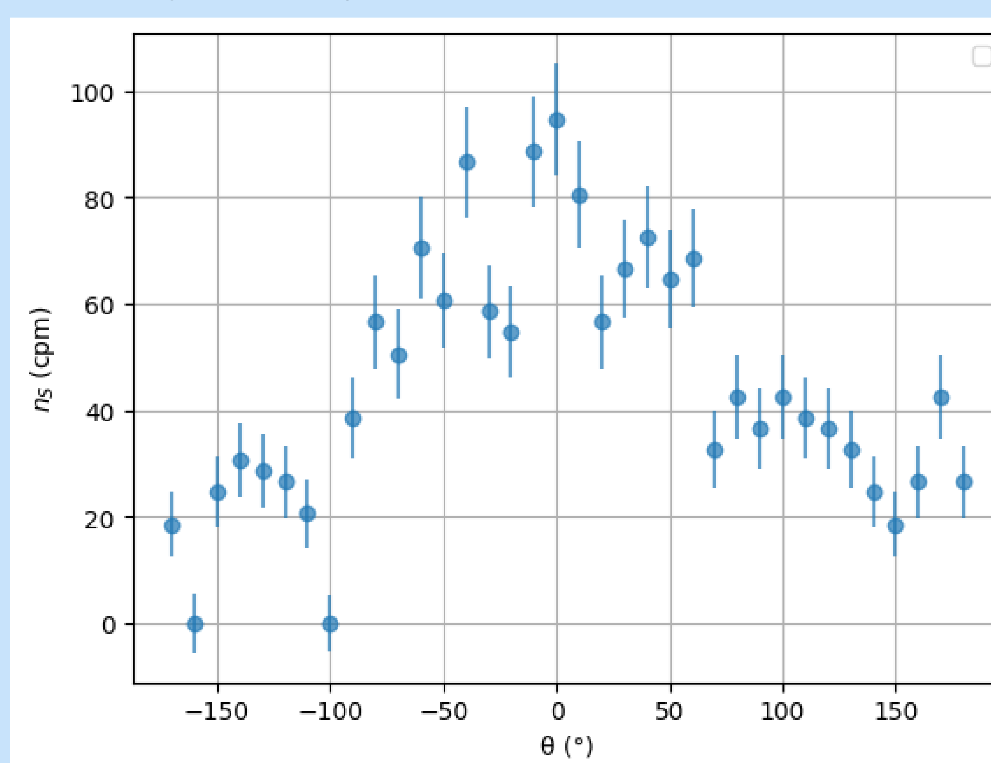
Figure 7. The net count rate of dots ( n_s ) depending on the detector rotation angle ( \theta )
