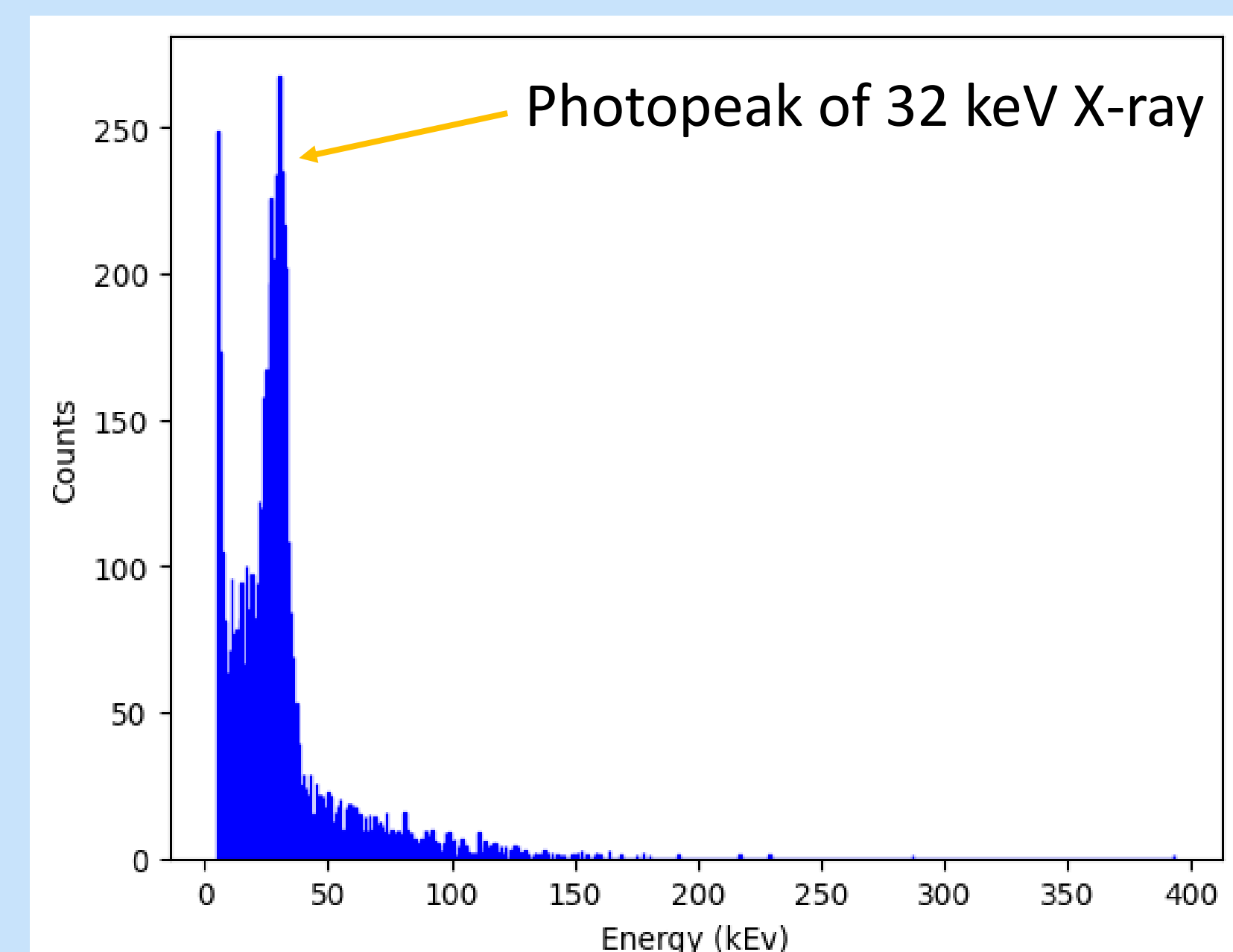
Figure 5. Histogram of dots' energy from ^{137}\text{Cs}
