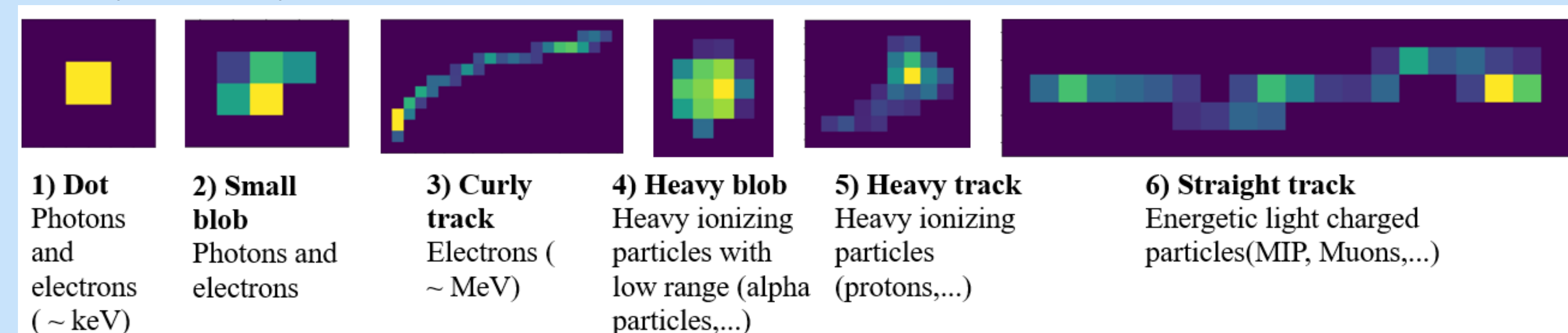
Figure 6. Six groups of radioactive clusters
