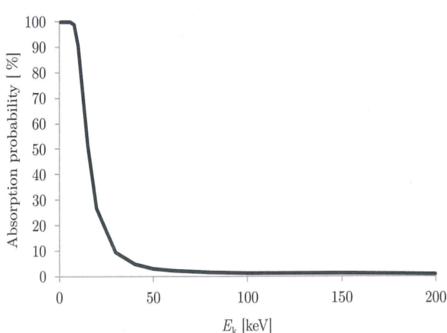
Figure 2. The photon absorption probability varies with energy [4]
