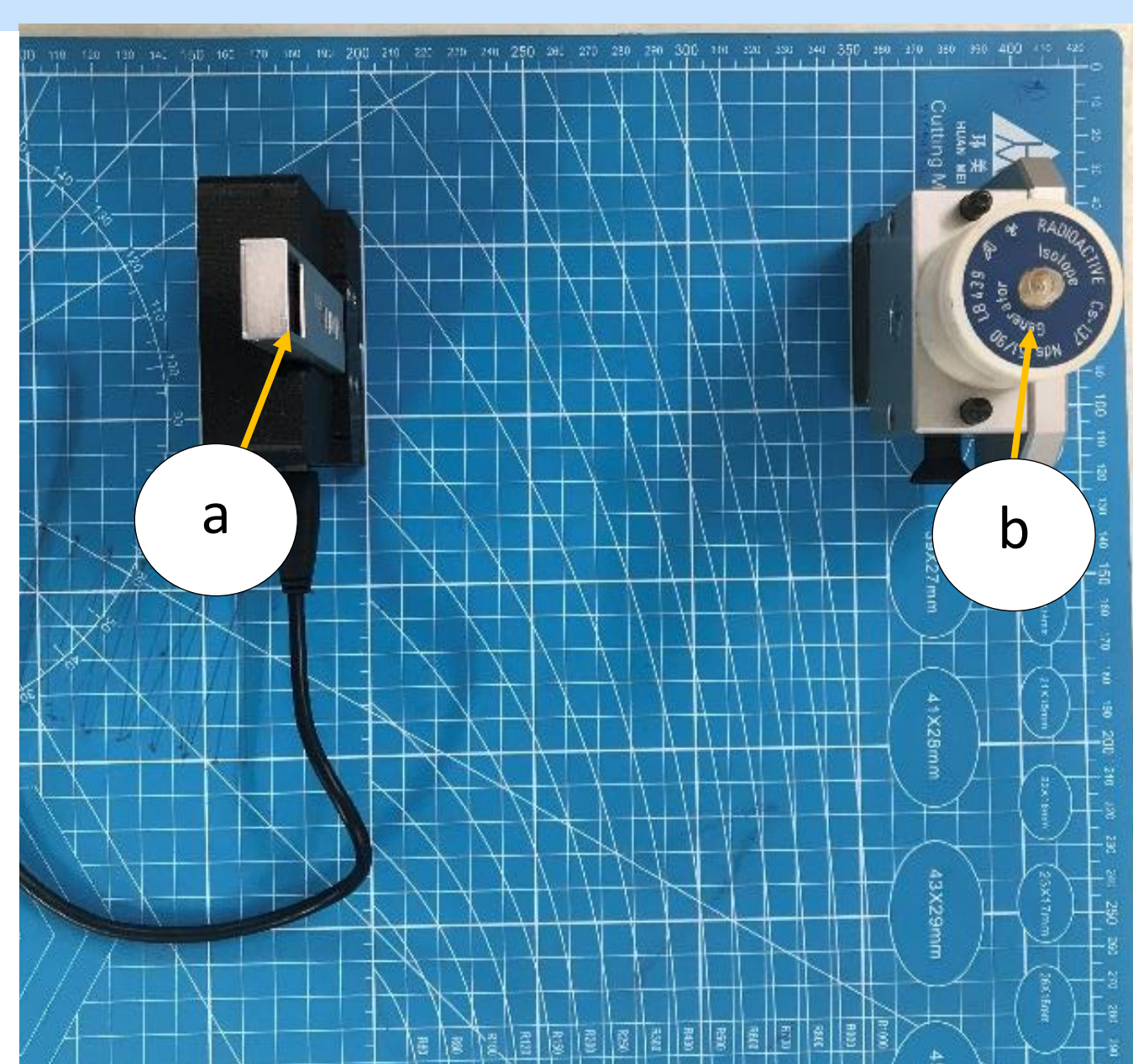
Figure 3. Experimental setups (top view): (a) is the Timepix and (b) is the ^{137}\text{Cs} source
