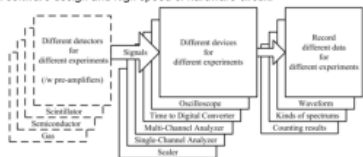
Fig. 1. Classic schemes for particle physics experiments
