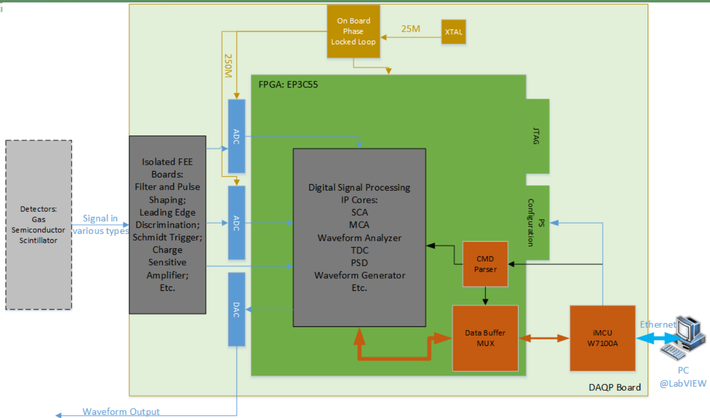
Structure of the DAQP System
