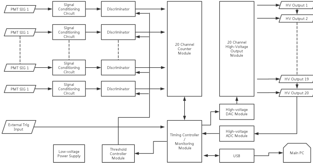
Fig.1 Schematic of the neutron flux DAQ system
