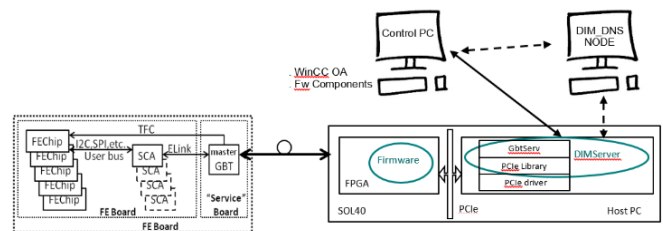
Fig 1. Architecture of the control system for the front-end electronics boards
