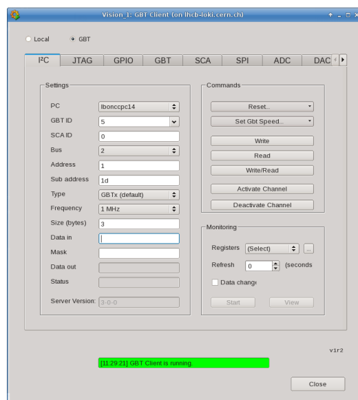
Fig 2. fwGbt GBT Client User Interface
