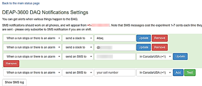
Fig. 10. Web page for notification settings. SMS or notification to cloud-based team collaboration tool.
