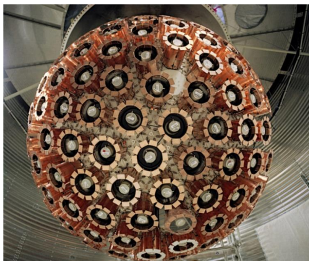
Fig. 1. DEAP detector sphere with 255 PMTs. Visible the PMTs and heat transfer Copper pads.
