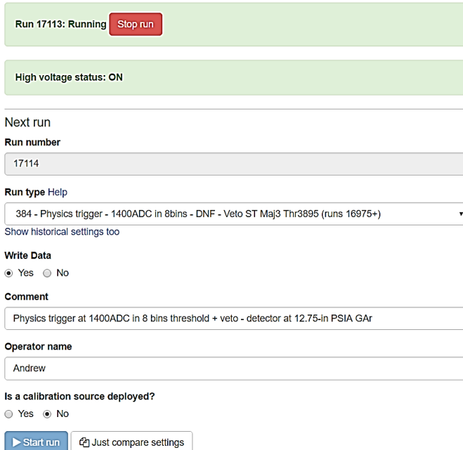
Fig. 11 Run control with run type selection provided by CouchDB.
