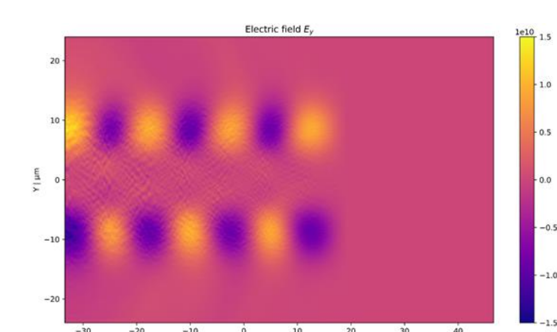
Transverse fields in the wakefield driven by two pulses.
