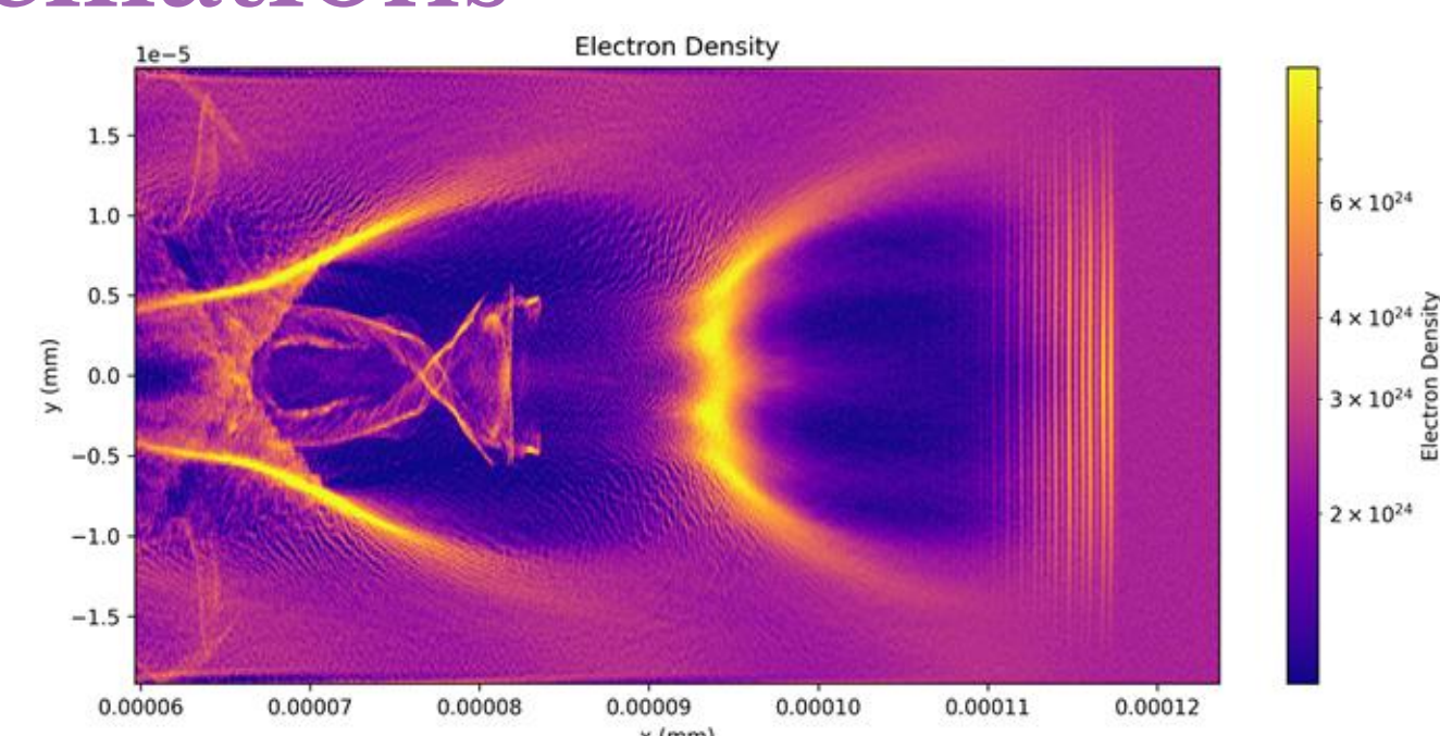
Particles injected into the wakefield
