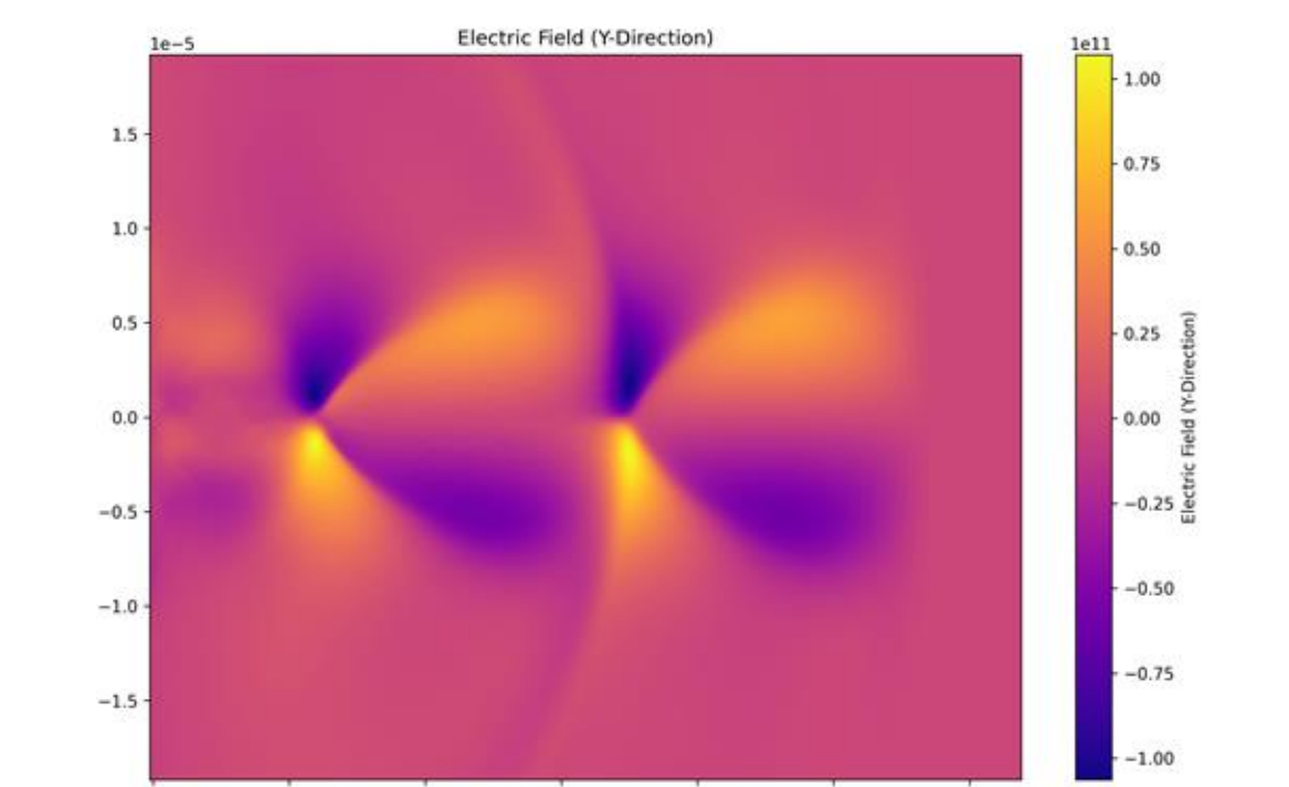
Transverse fields in the wakefield driven by a single pulse.
