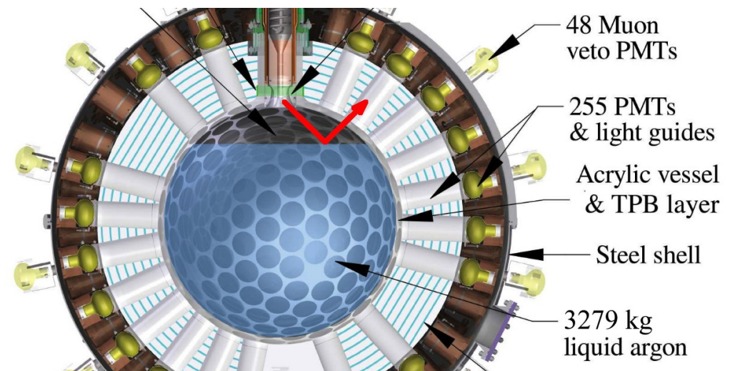
UV photon reflection at the liquid argon surface 14
