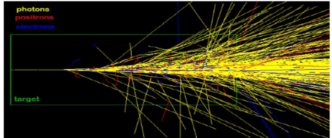
Massive shower in a tungsten cylinder (outlined in green) produced by a single 10 GeV incident electron.
