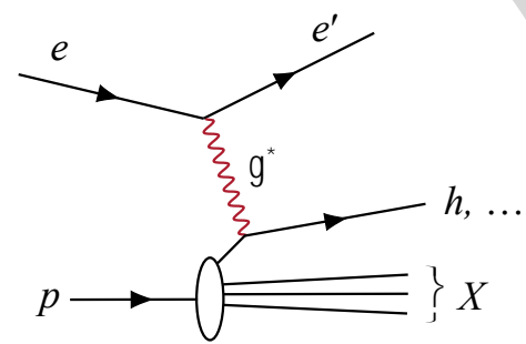
Semi-Inclusive DIS
