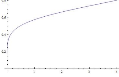
Figure 2.2: H as a function of k (for particles with finite mass and large but finite Energy)
