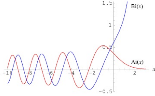
Figure 2.1: Airy functions and the zeroes [35]
