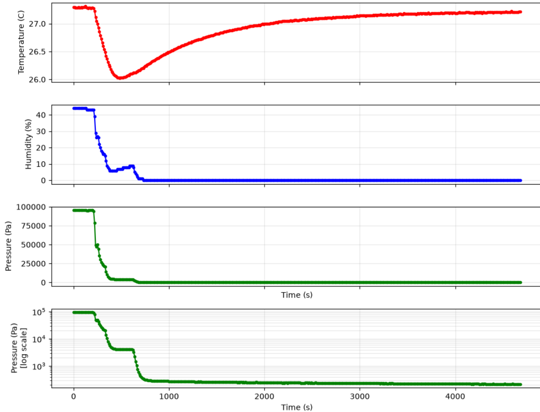
BME280 Sensor Readings Over Time
