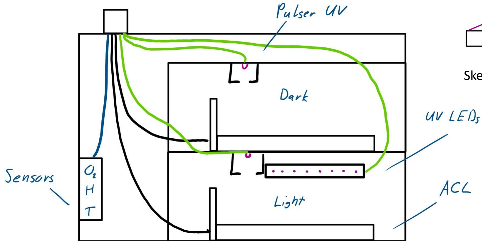
Sketch of vacuum-box with experiment setup
