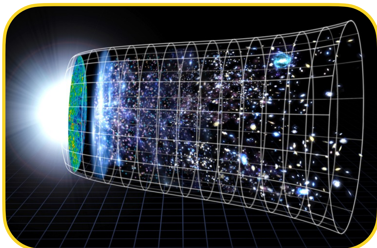
Contributors to reionization?
