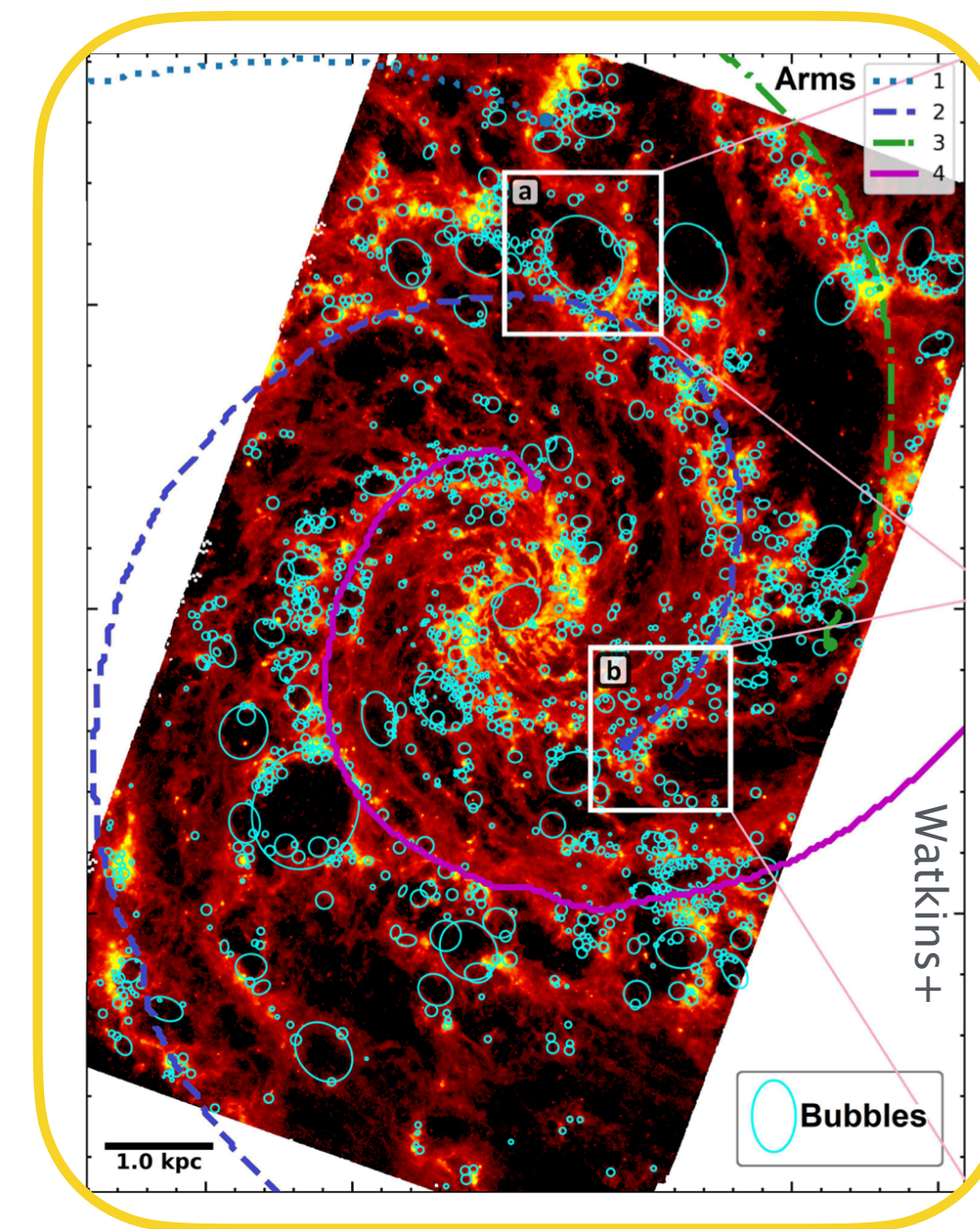
Interplay with galactic ecosystems
