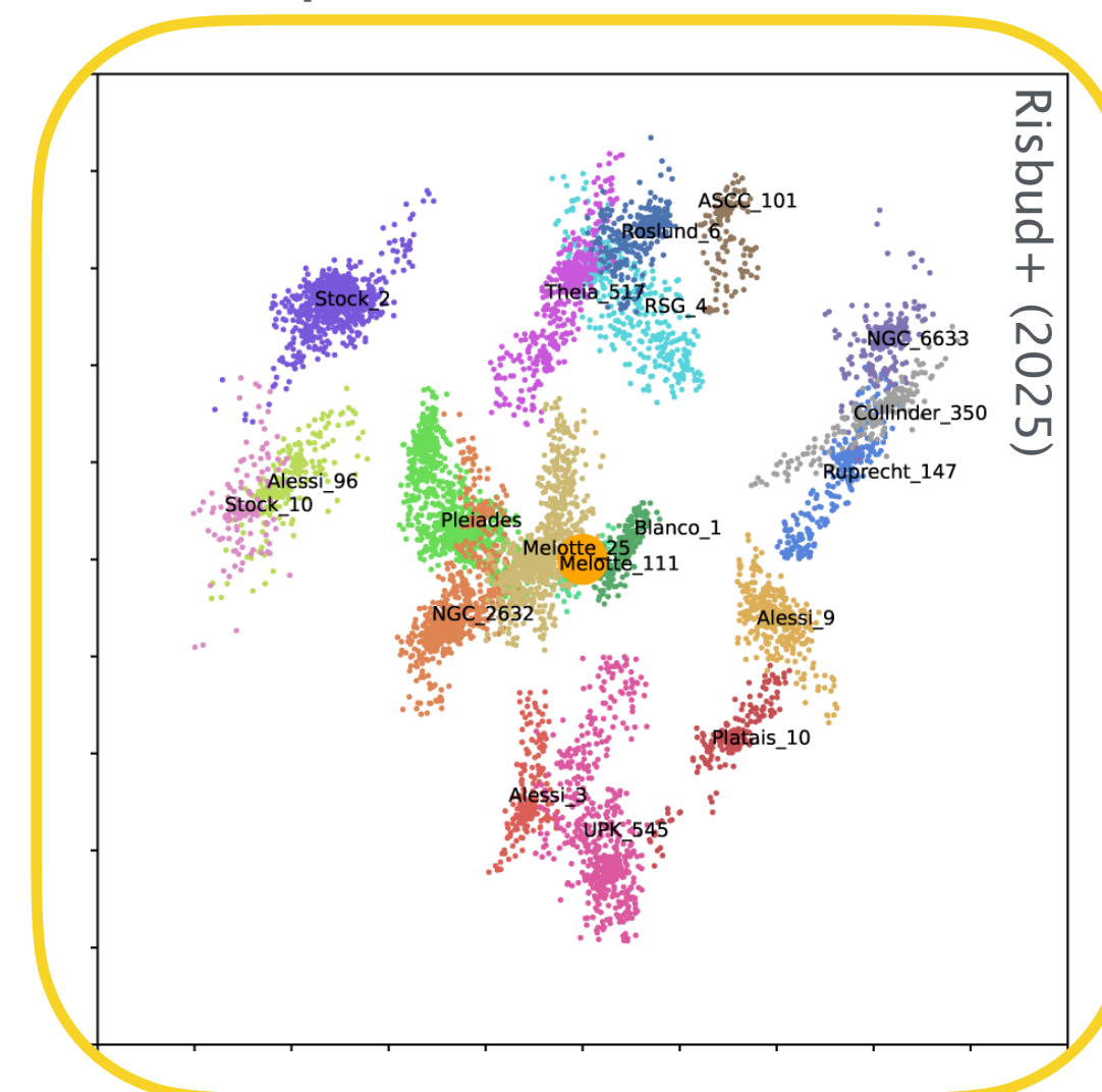
Disruption of star clusters
