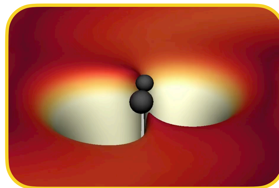
Compact objects and gravitational waves
