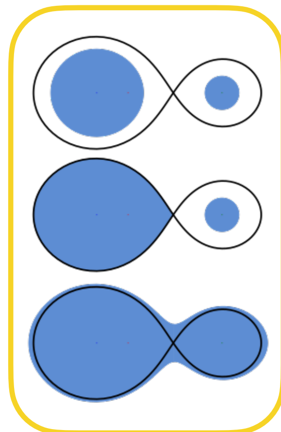
Binary stars
