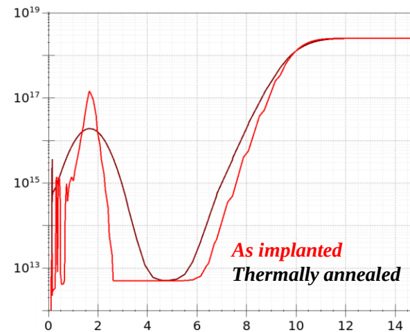
An example of doping profile from 11 B implantation in <100> Si, as implanted and after thermal annealing
