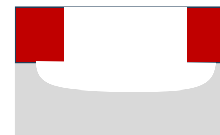
Poor anisotropy: round sidewalls
