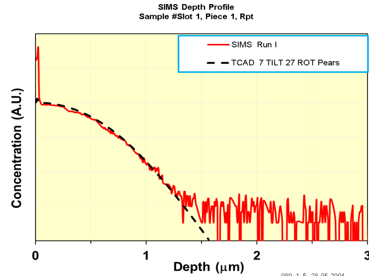
SIMS and Pearson IV distribution – 31P on \langle 100 \rangle Si
