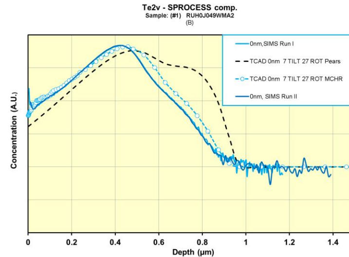
SIMS, Pearson IV distribution and MC run – 11B on \langle 100 \rangle Si
