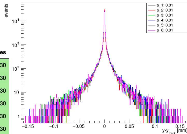
LocalResidualsY
