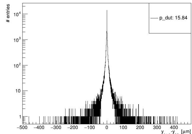
residualsY
