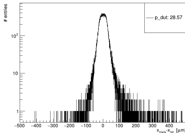
residualsX
