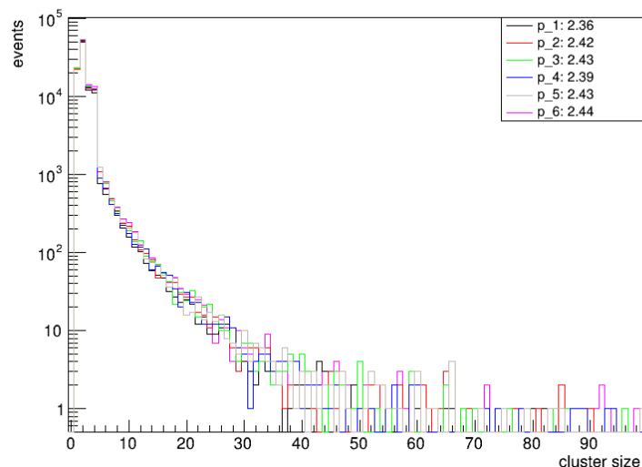
clusterSize
