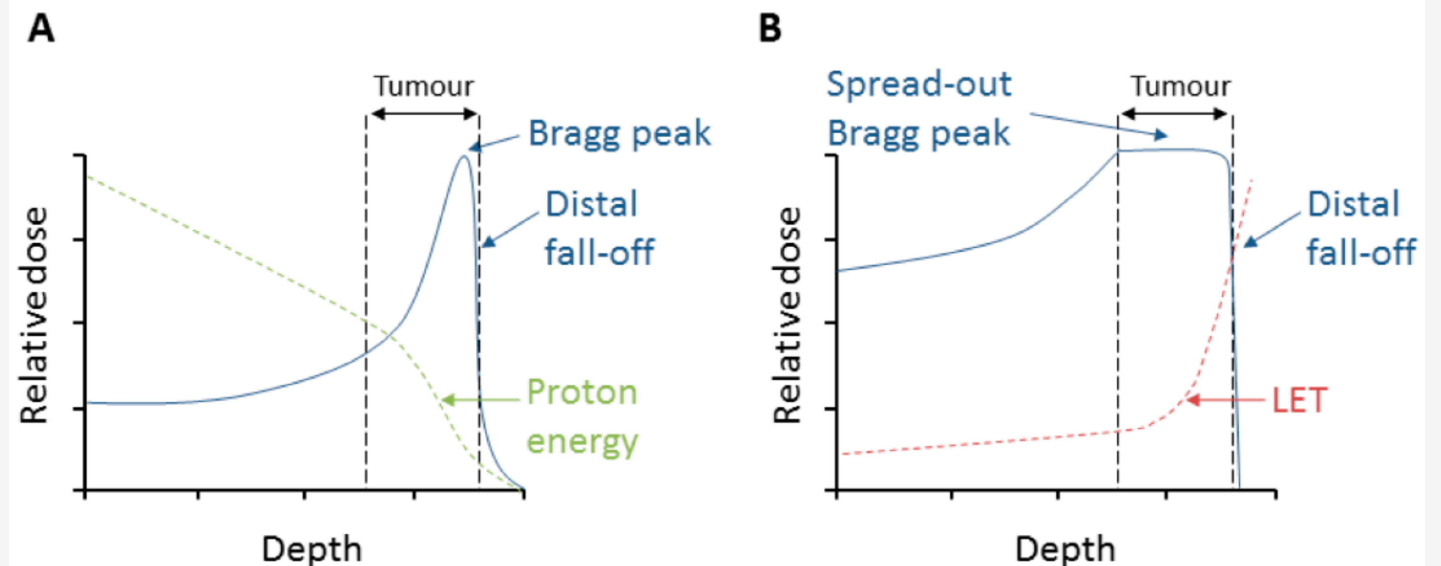
Figure 1. Depth–dose distribution of protons and relationship to energy and linear energy transfer (LET). (A) An unmodulated (pristine) Bragg peak produced by a proton beam. (B) Spread-out Bragg peak (SOBP) from several modulated proton beams.
