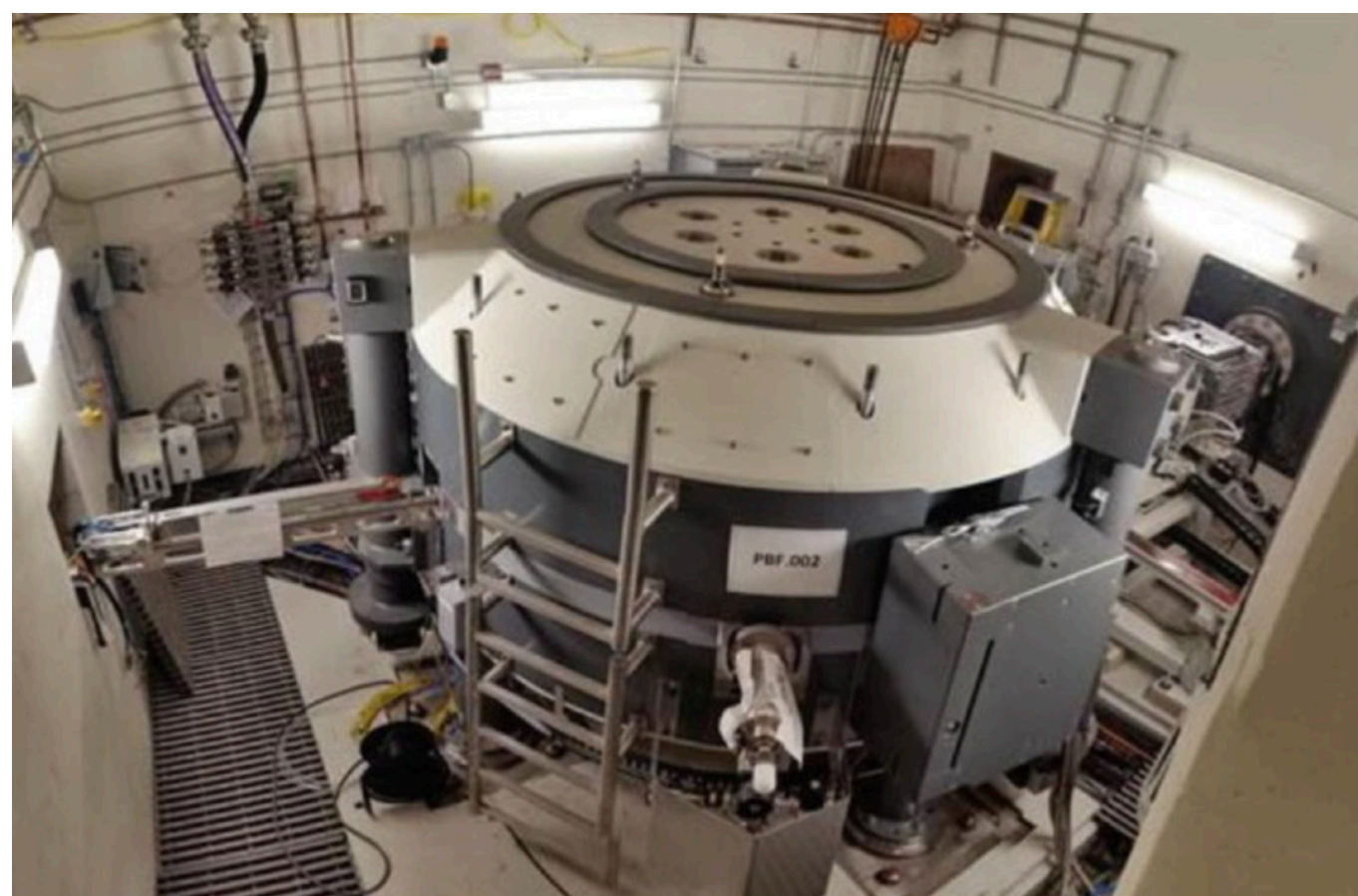
IBA Proteus one superconducting cyclotron (230 MeV protons)
