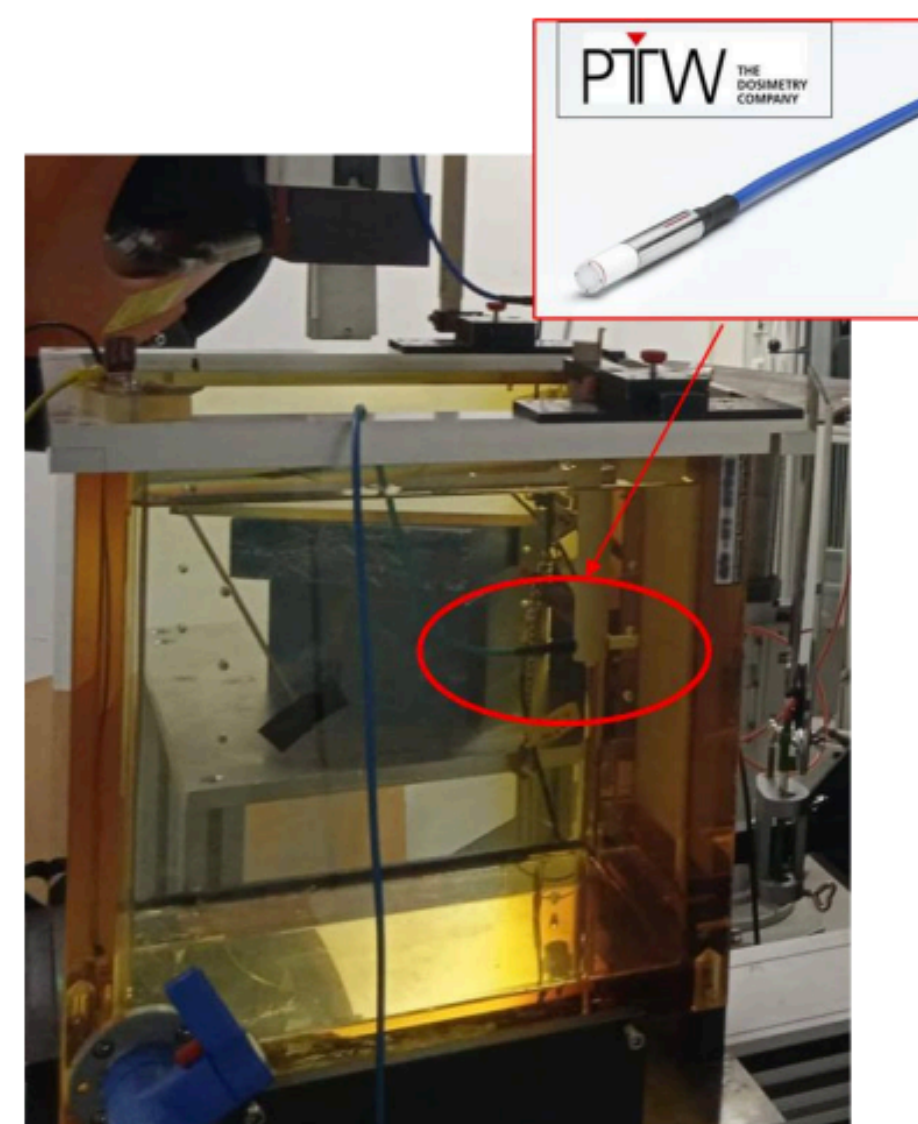
SiC diode in water phantom at PTB
