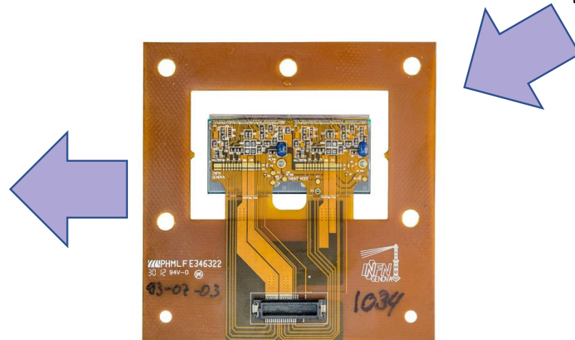
ATLAS IBL – pixel dual- module (50 x 250 \mu\text{m}^2 )
