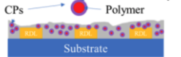
(b) ACF Bonding
