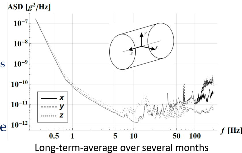
ATLAS ID – measured ASD spectrum
