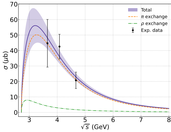
FIG. 3: The calculated total production cross section for the K_3^*(1780) state is presented, along with comparisons to experimental data. The experimental data are taken from Refs. [14–16]. All error bands and the solid lines within them correspond to results obtained with the cutoff parameter set to 1.5 \pm 0.2 GeV.
