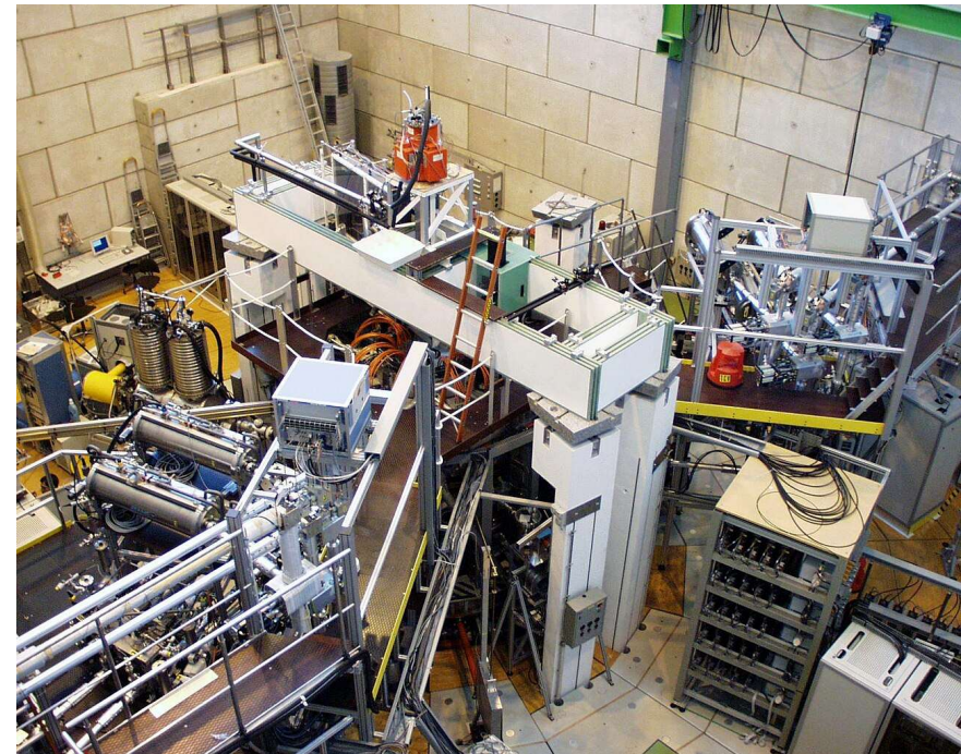
Tokamak TCA, Lausanne 1983
