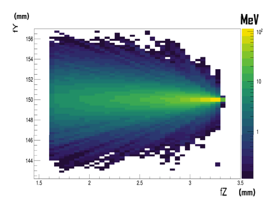
Alpha spatial energy deposition in drift gap
