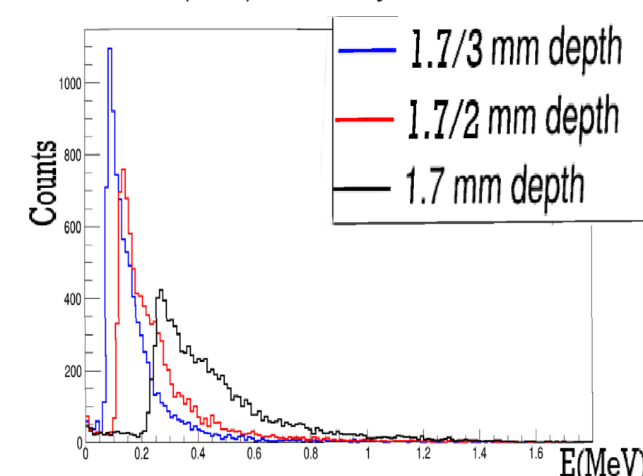
Alpha Energy Deposition vs Drift Gap
