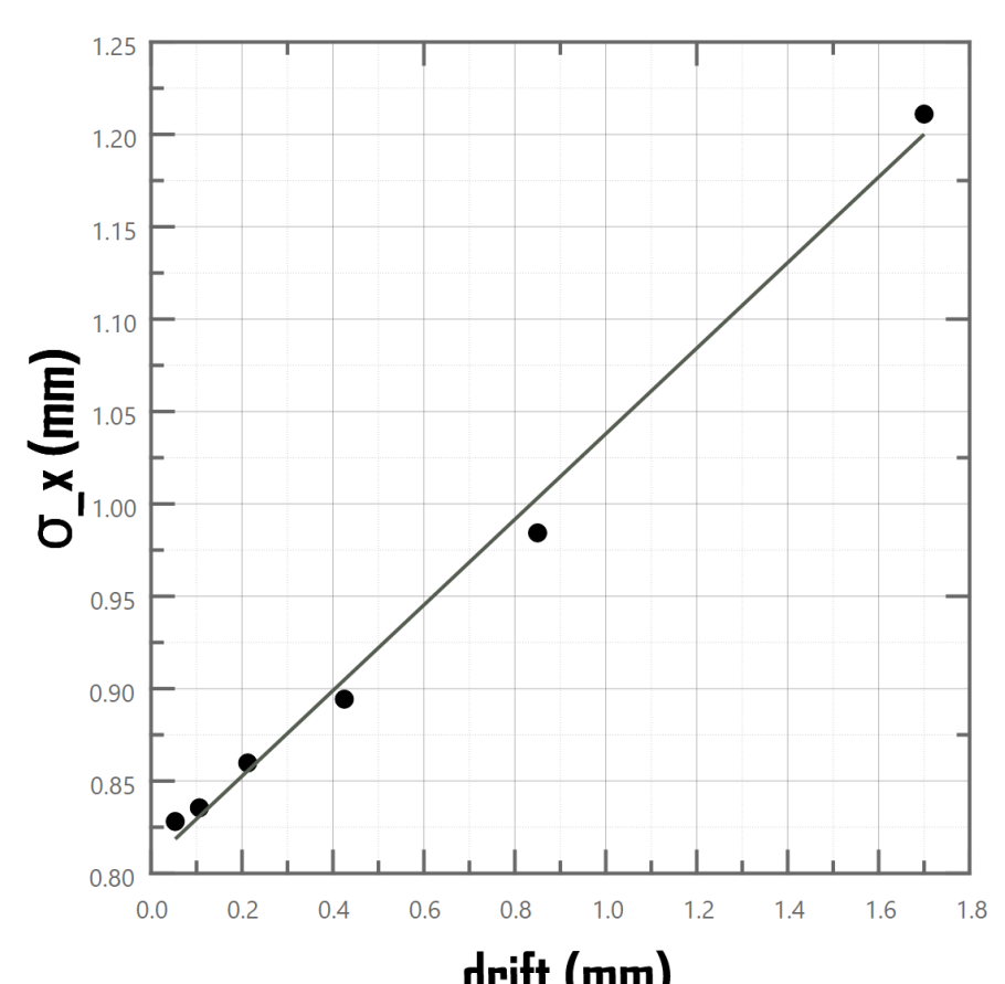
Spatial Resolution vs drift gap size
