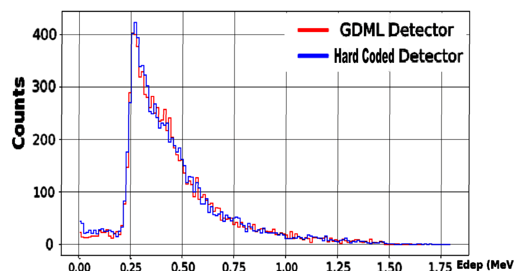
Alpha Edep: GDML vs Hard-Coded Geometry
