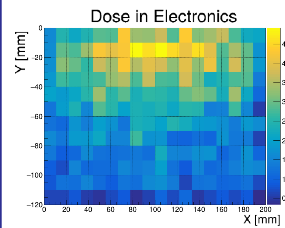
1. Single Slab
