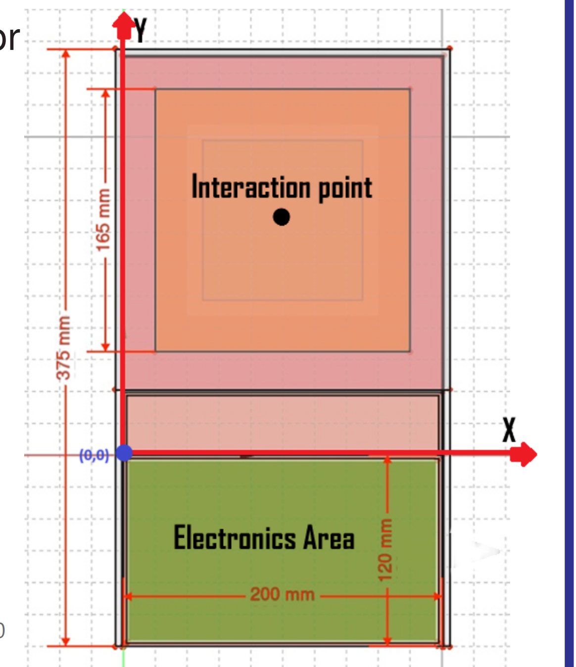
Detector Geometry
