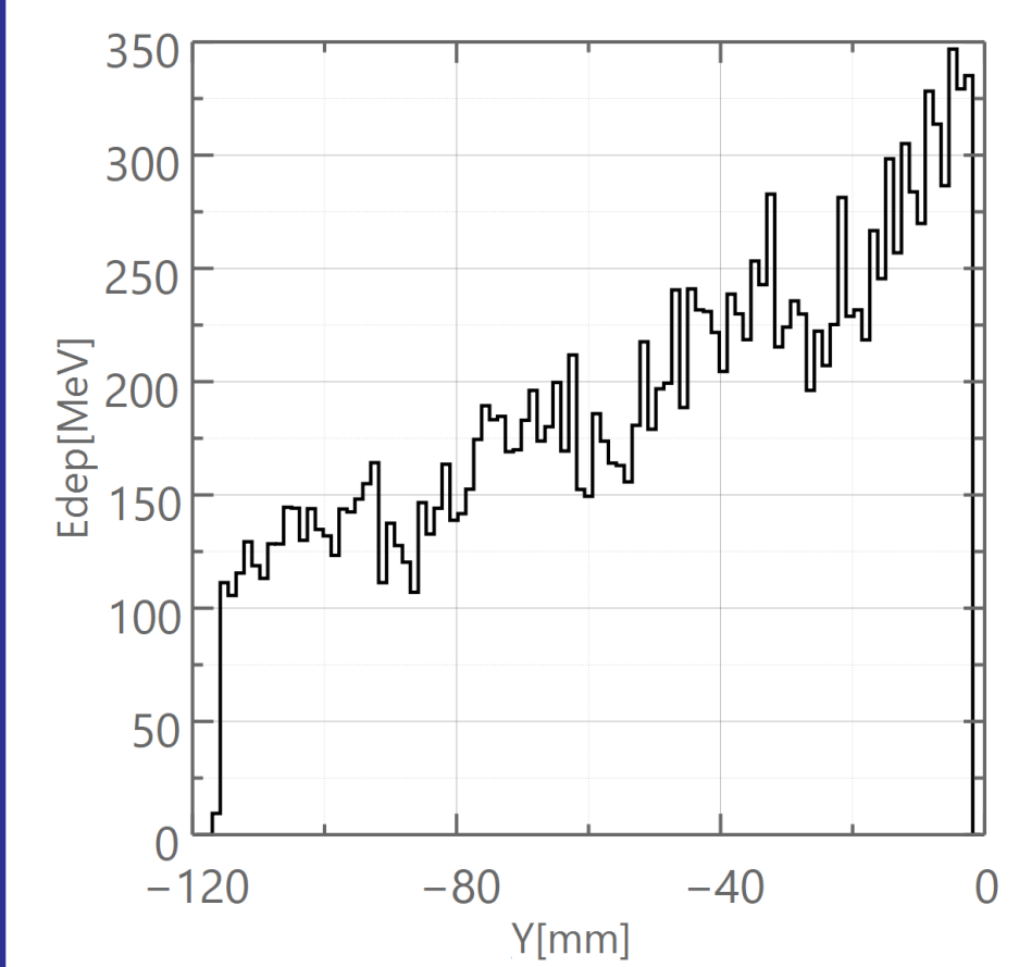
Dose decreases toward lower Y positions
