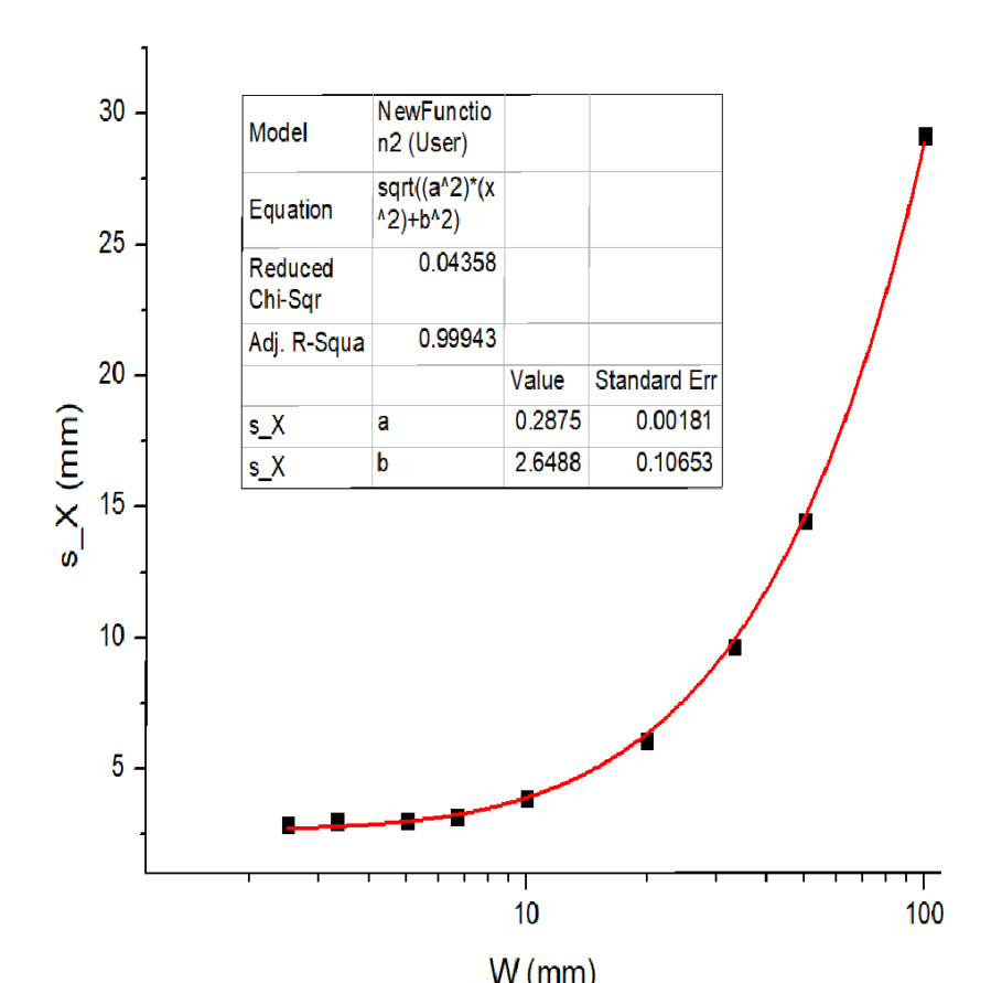
Spatial Resolution vs Strip Width W
