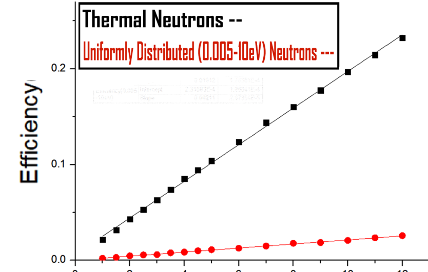
^{10}B(n,\alpha) efficiency vs thickness
