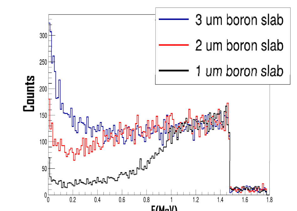
Emergent Alpha Energy vs B_4C Thickness
