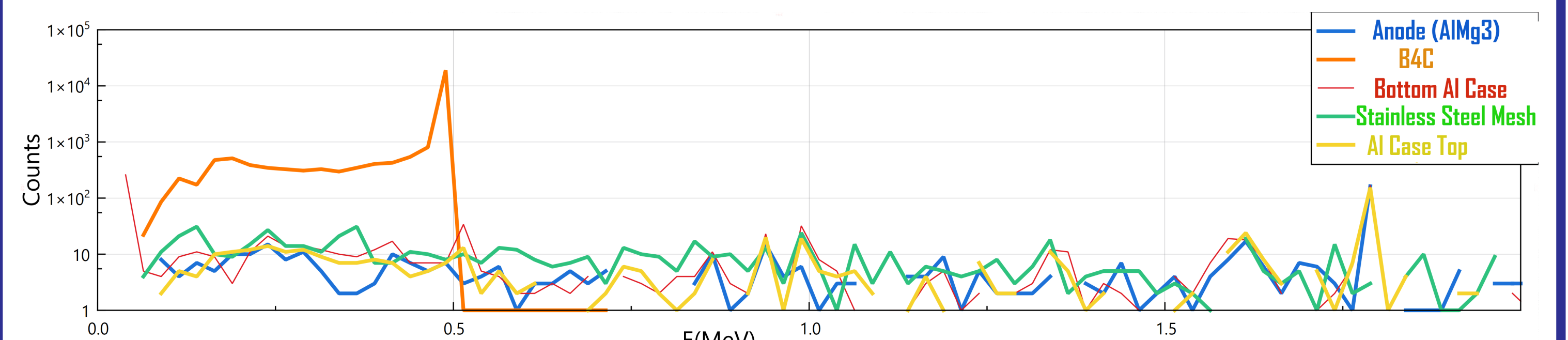
Secondary \gamma -ray interaction Energy spectrum grouped by detector volume
