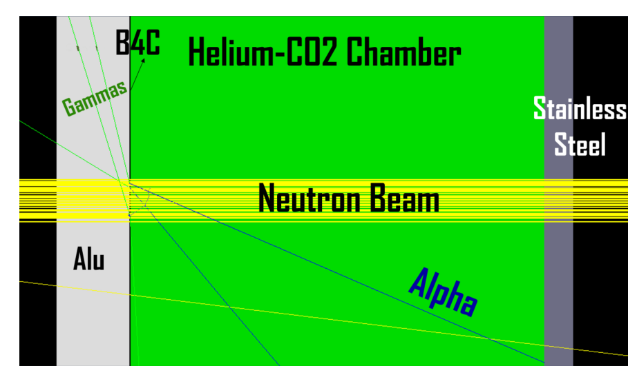
^{10}B(n,\alpha)^7Li interaction and the Drift Gap
