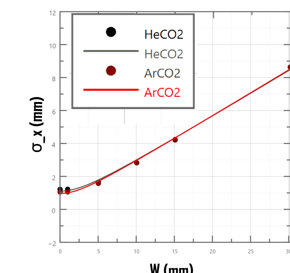
HeCO 2 /ArCO 2 Spatial Resolution vs Strip Width W
