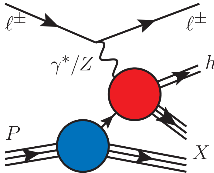
Semi-inclusive DIS
