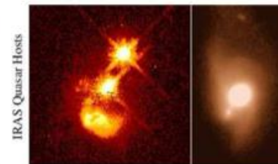
(e) "Blowout"
