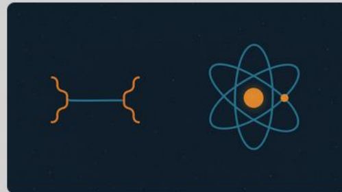
Quantum Field Theory
