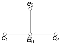
Fig. 1. The O(8) Diagram
