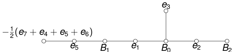
Fig. 6. The E_8 Dynkin Diagram
