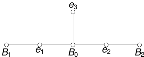
Fig. 3. The E_6 Diagram
