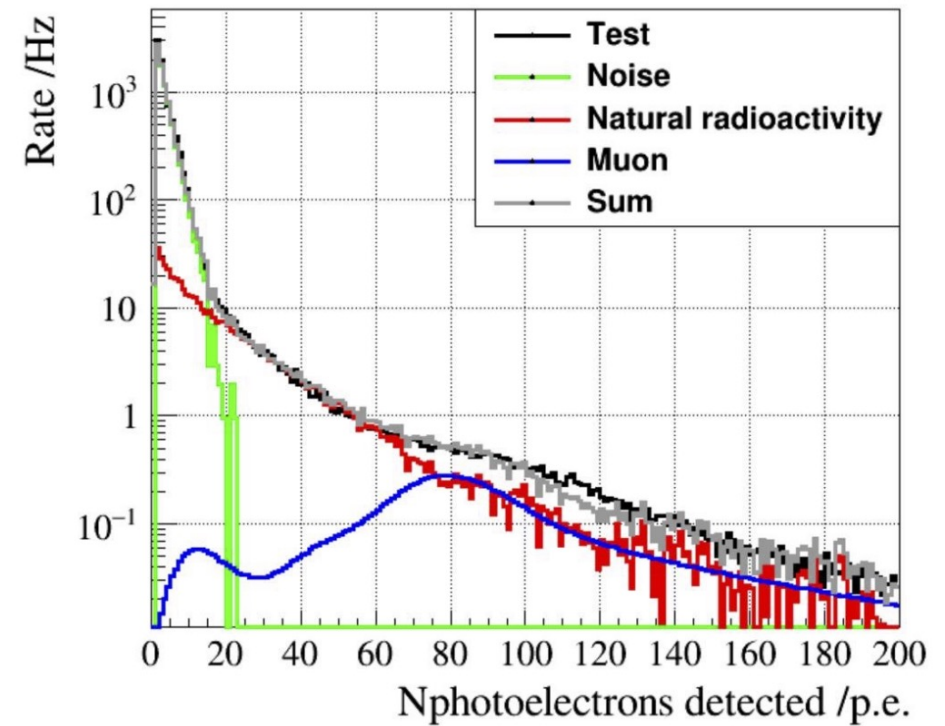
(b) NNVT PMT fitted curves
