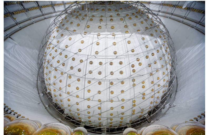
JUNO Collaboration
