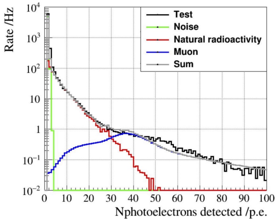
(a) HPK PMT fitted curves
