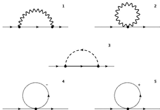
Figure 4: One-loop Feynman diagrams contributing to the two-point Green's functions \langle A_+ A_+^\dagger \rangle and \langle A_-^\dagger A_- \rangle .
