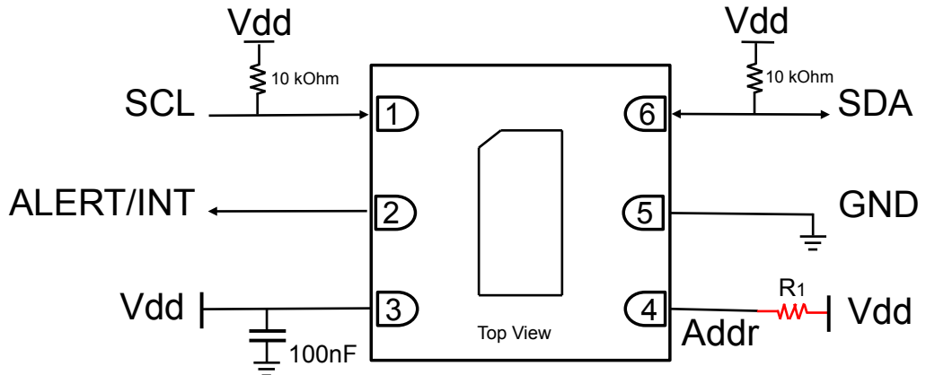
Figure 6. STTS22H electrical connections (pull-up on Addr)
