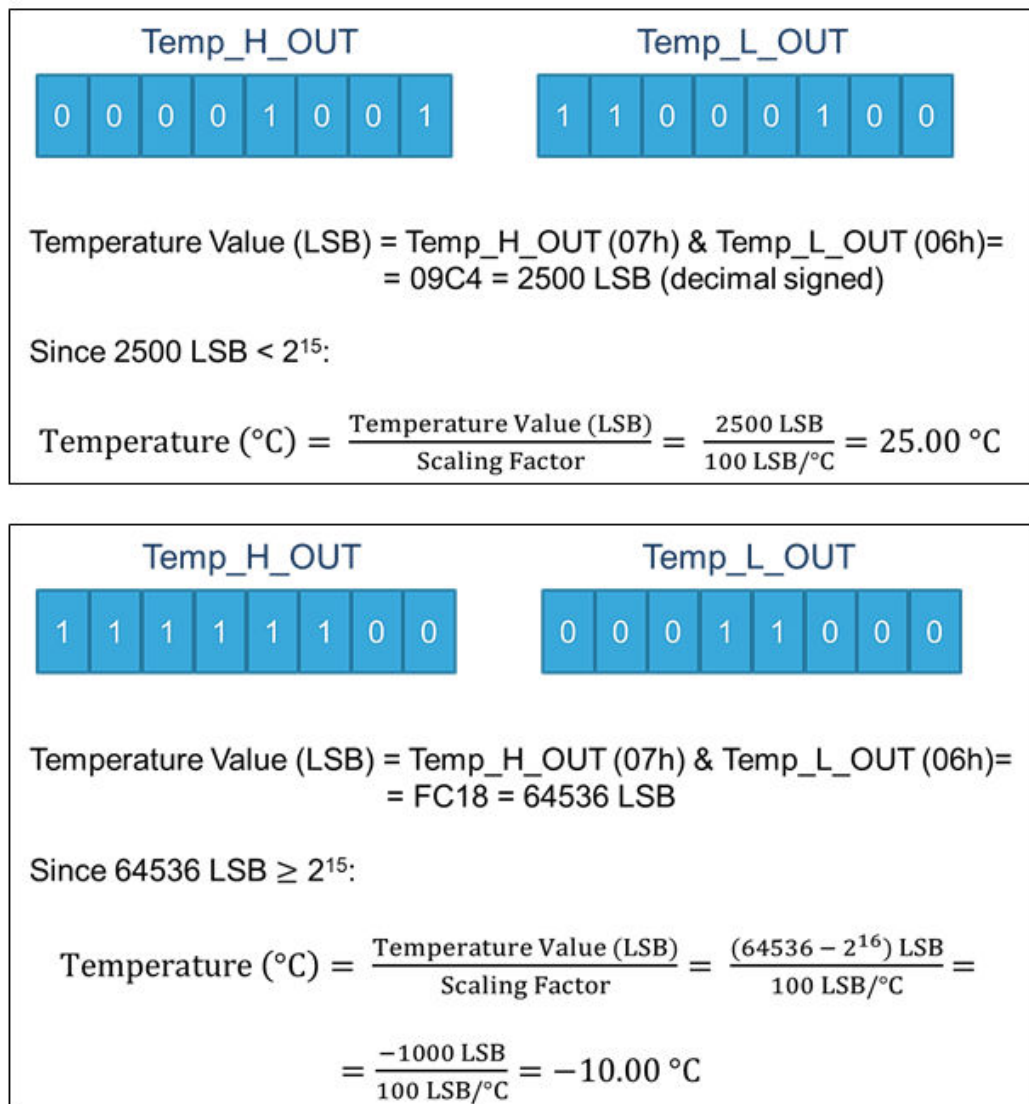
Figure 7. Temperature readings
