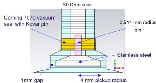
Fig 27: A cross-section of the initial pickup model used in thermal studies.
