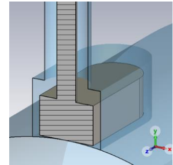
Fig 23: Pill-shaped button with ratio 4 modelled in CST, sliced at z=0 .
