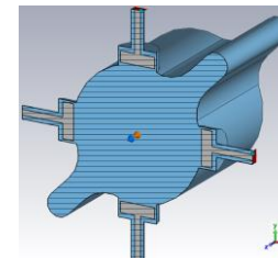
Fig 2: A simplified BPM model in CST, with FCC-ee beampipe.
