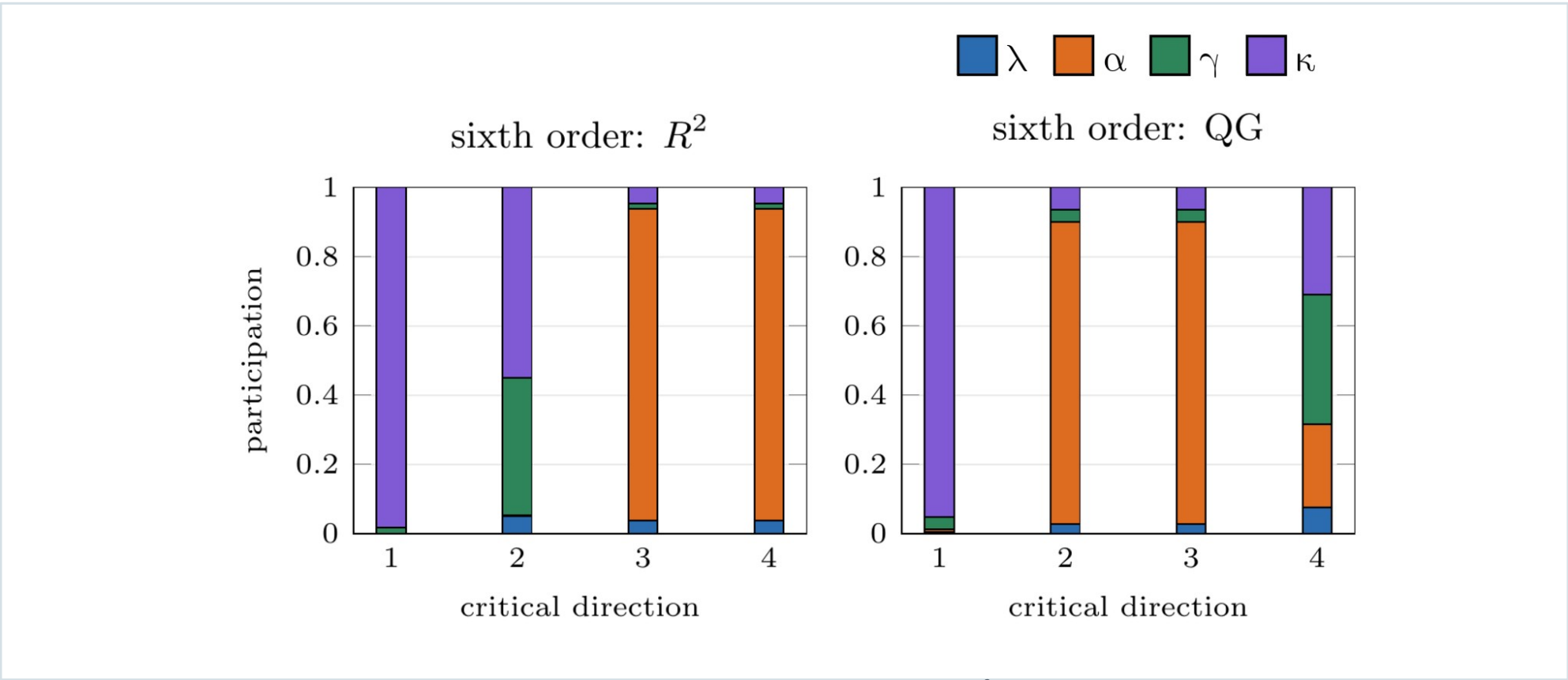
Sixth-order eigendirection participation at R^2 and QG
