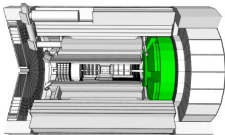
The dual-radiator Ring Imaging Cherenkov detector in ePIC [11].
