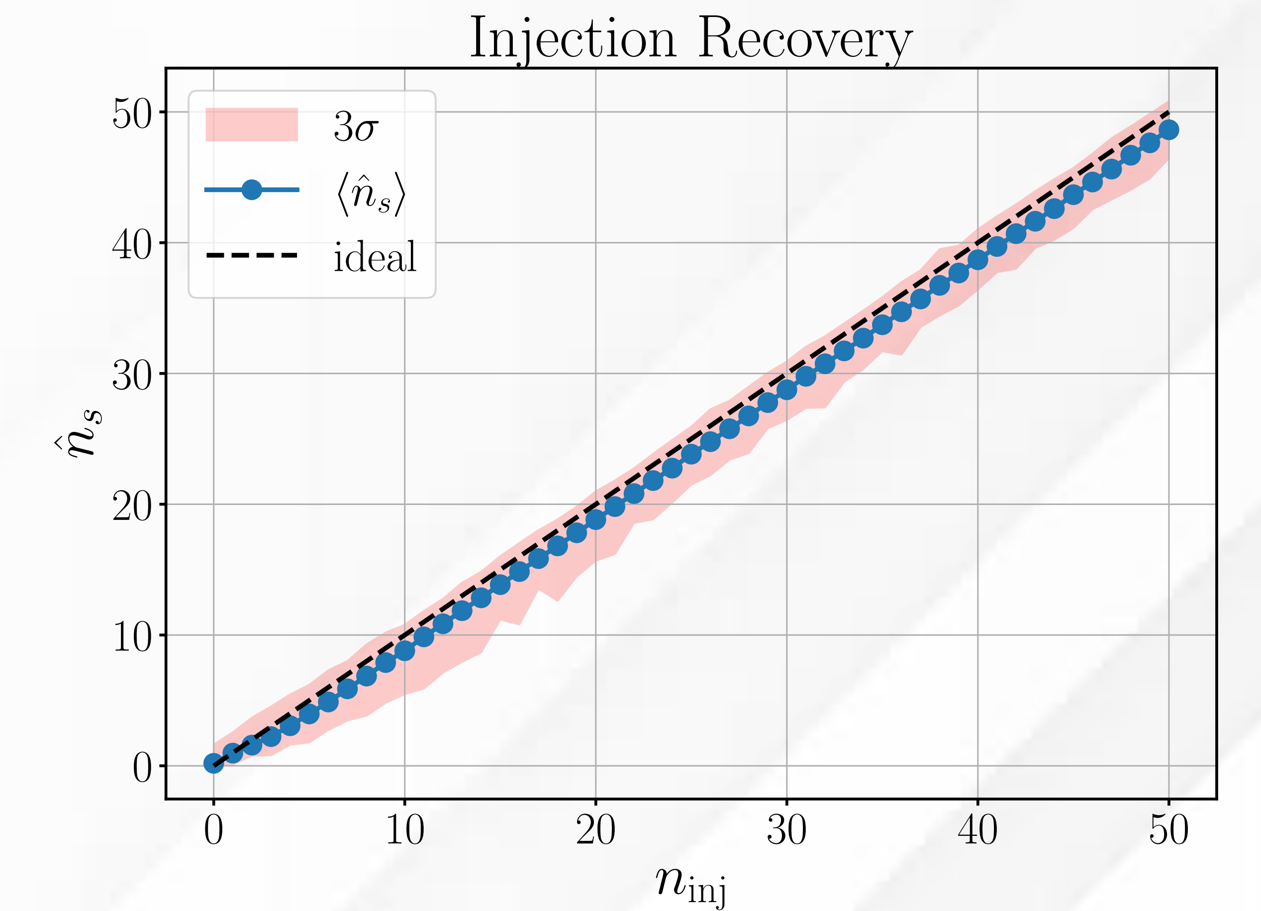
Figure 5: Recovering the injected signal neutrinos.
