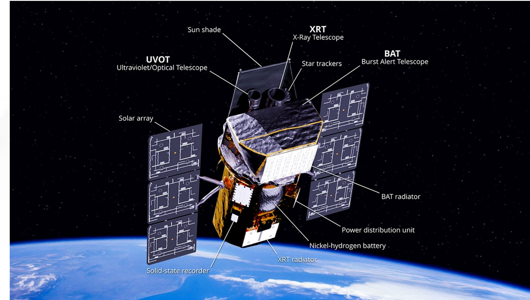
Figure 3: An artist's concept of the Neil Gehrels Swift Observatory.
