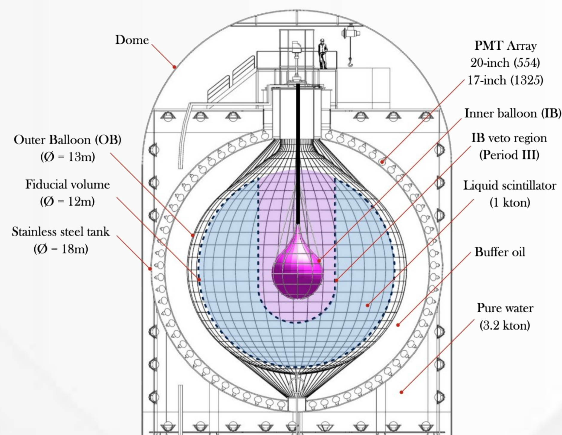
Figure 2: The KamLAND detector
