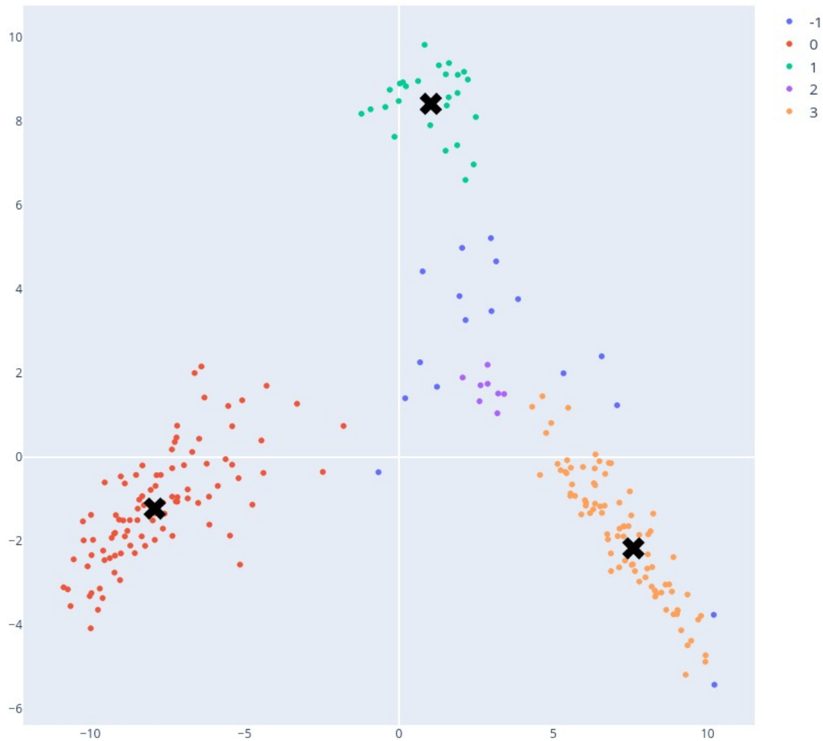
PCA reduction. HDBSCAN clustering on reduced data
