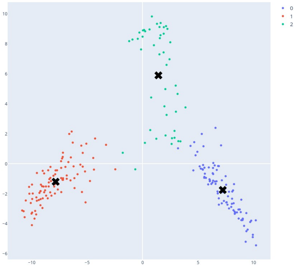
PCA reduction. K-means clustering on reduced data
