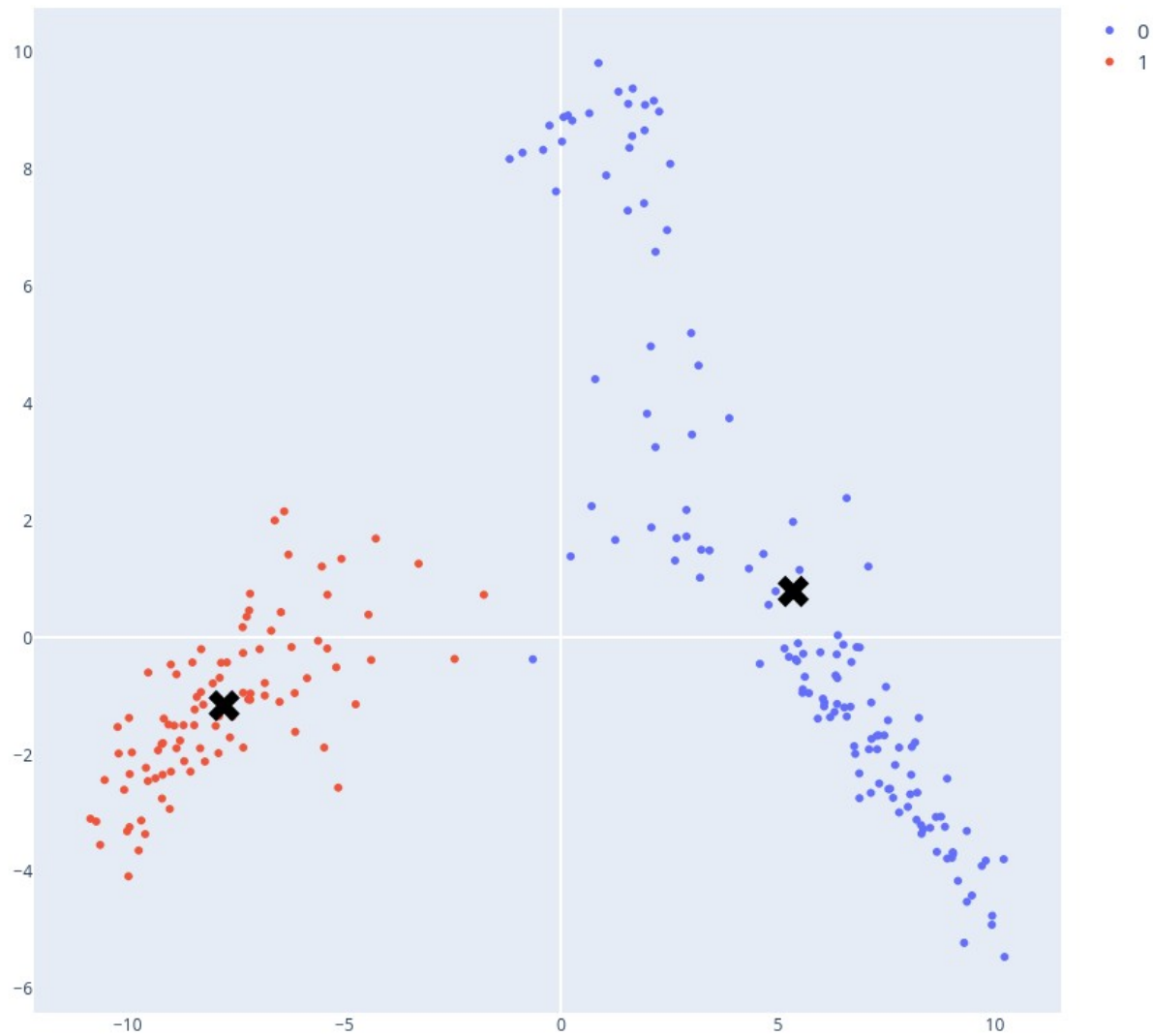
PCA reduction. K-means clustering on high dimensional data
