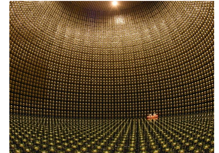
HYPER-K
