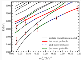
with a bare baryon
