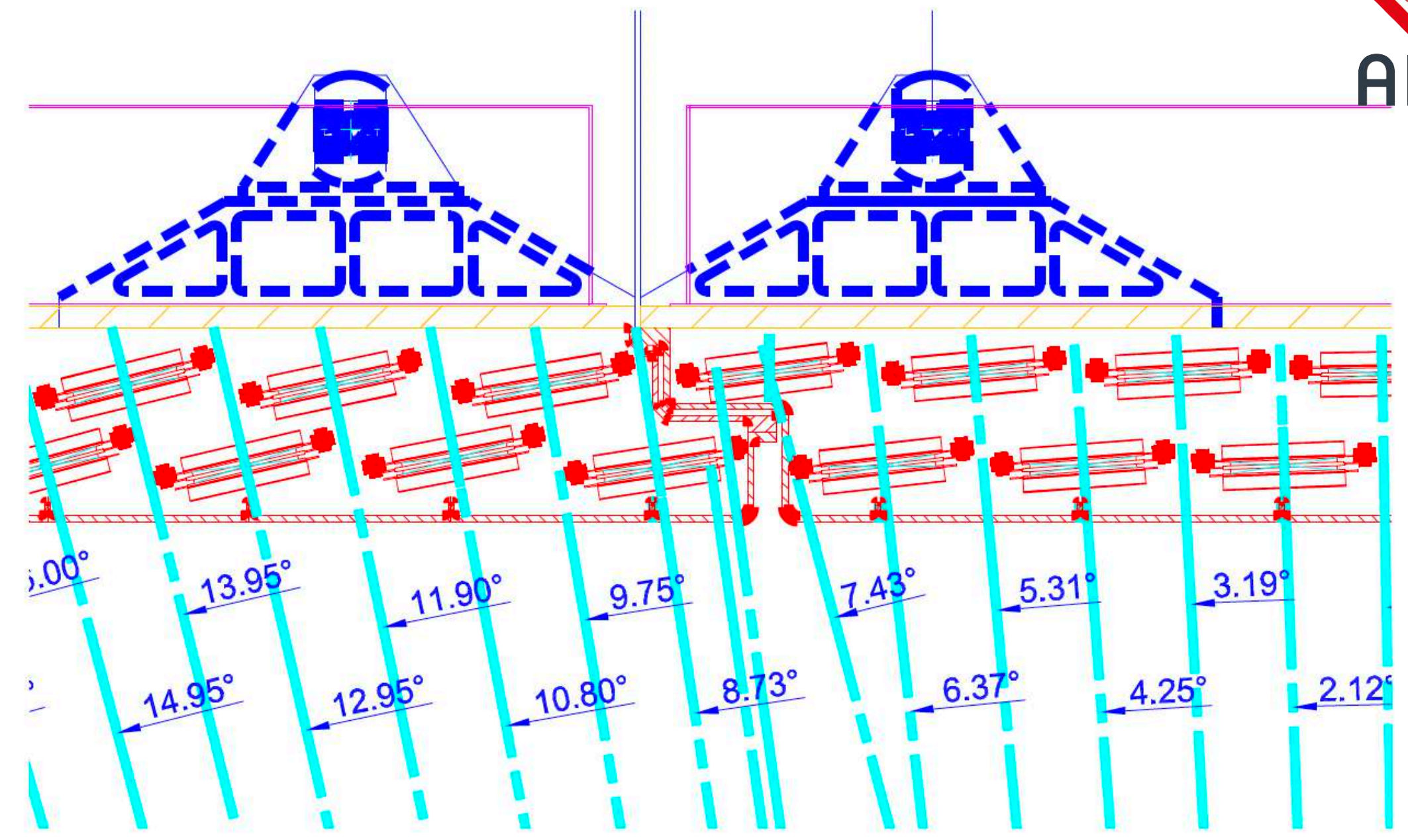
Figure 2.9: Detail of the overlap region between two modules and strip positioning. R. Preghenella - PhD thesis
