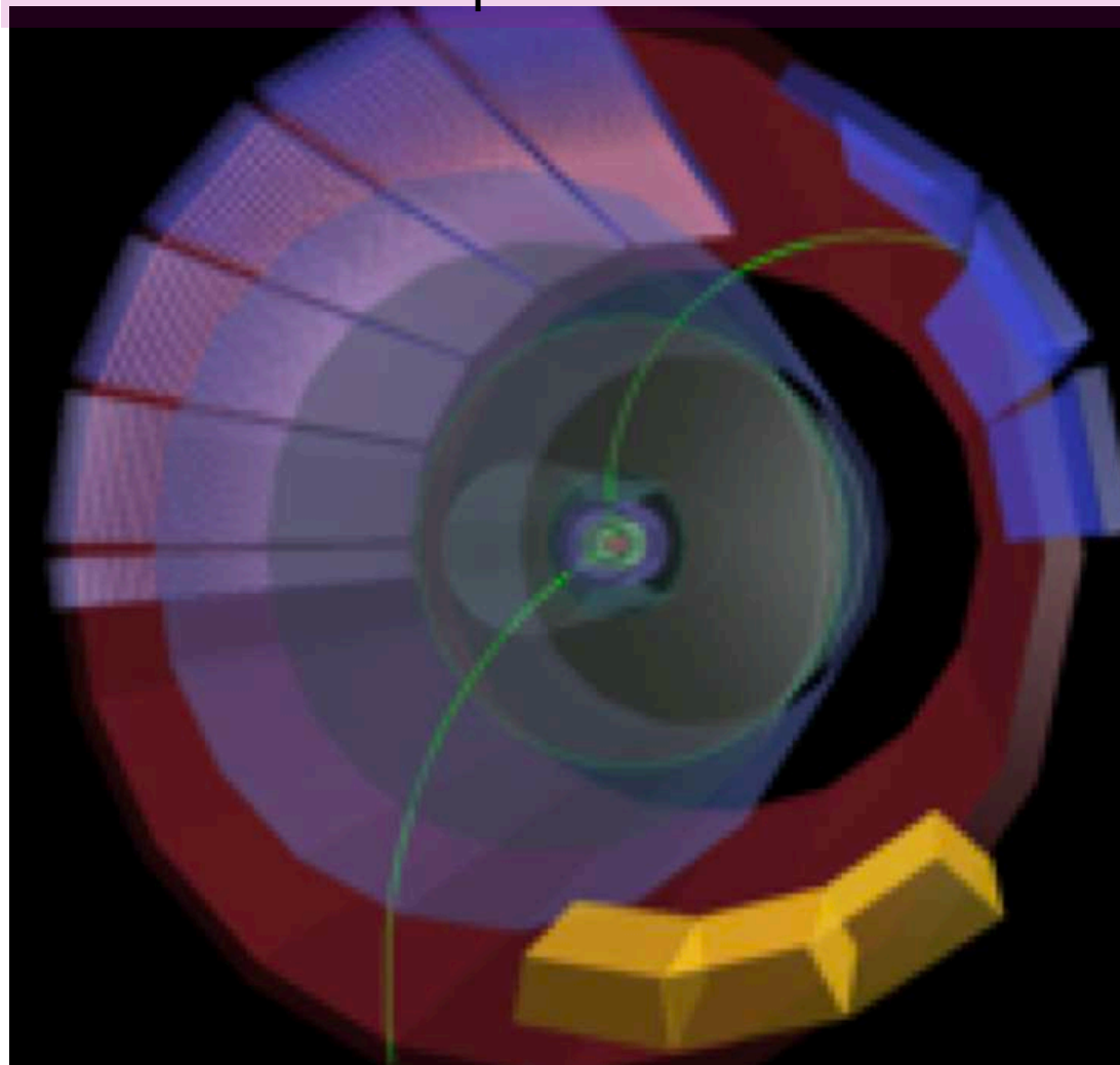
Ultra-Peripheral Collision
