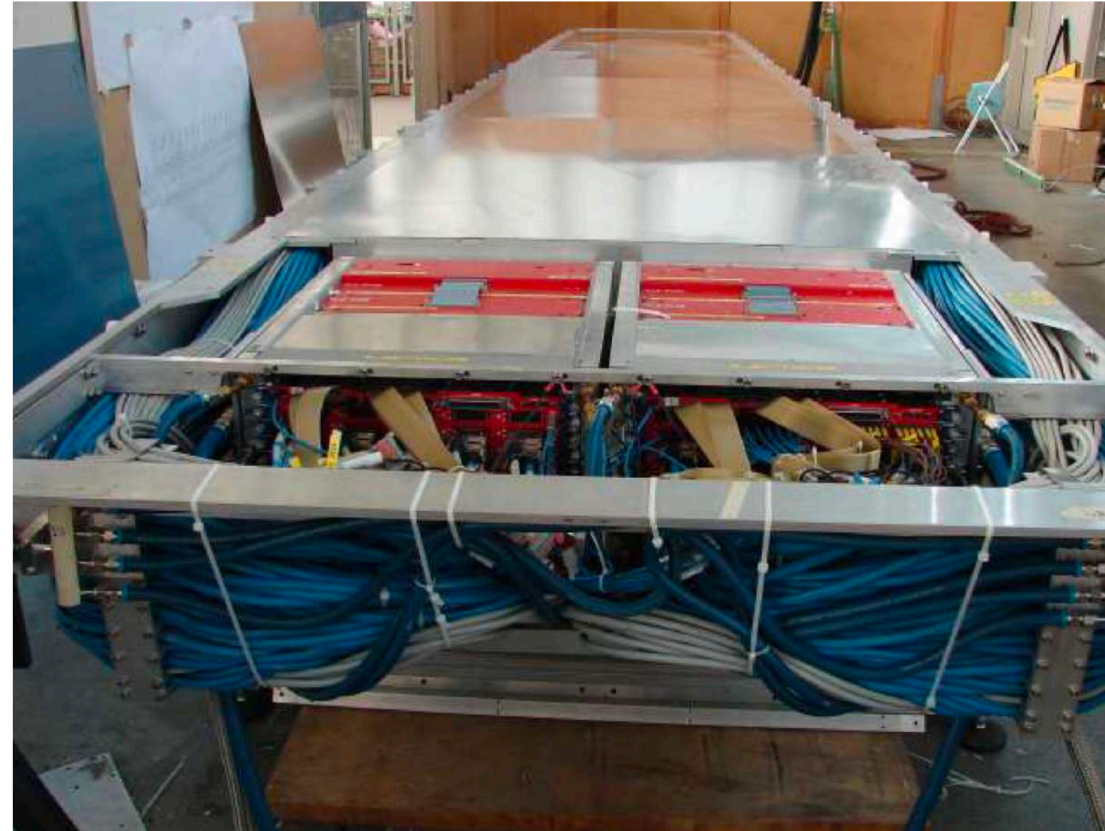
Photo of a fully assembled supermodule
