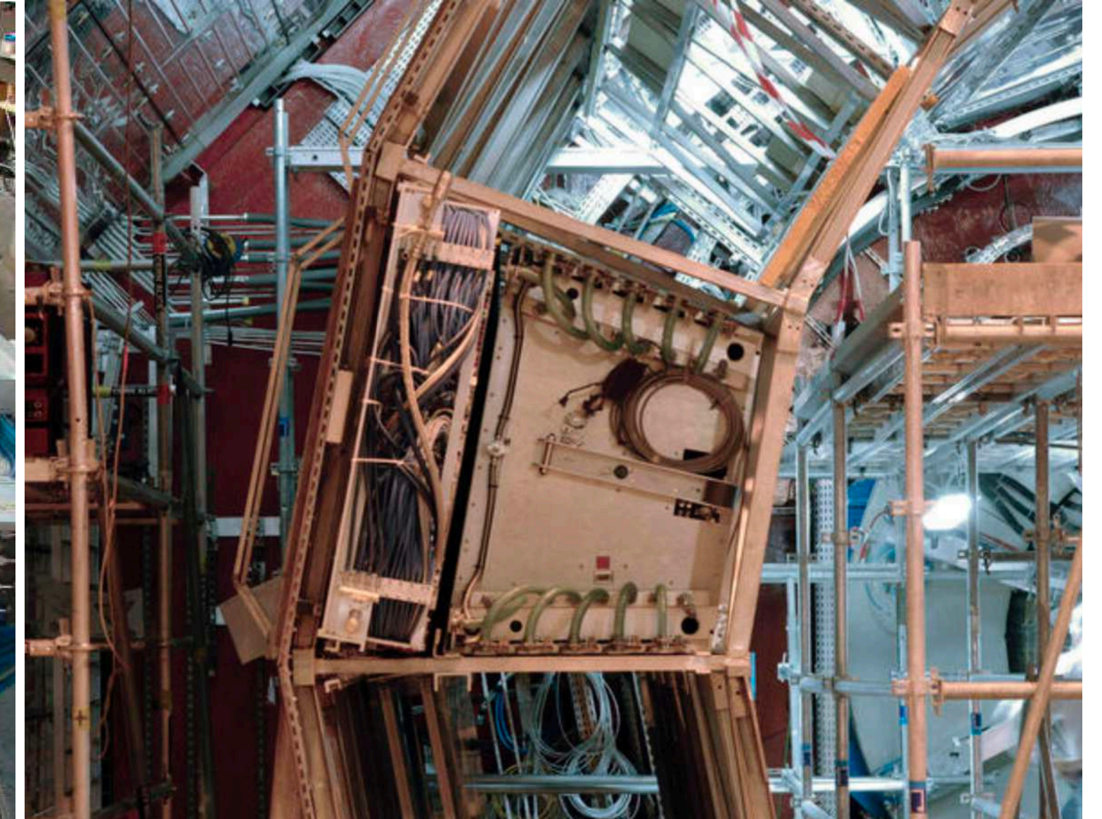
Two supermodules of the Time of Flight (TOF) and of the Transition Radiation Detectors (TRD) installed in their final position.
