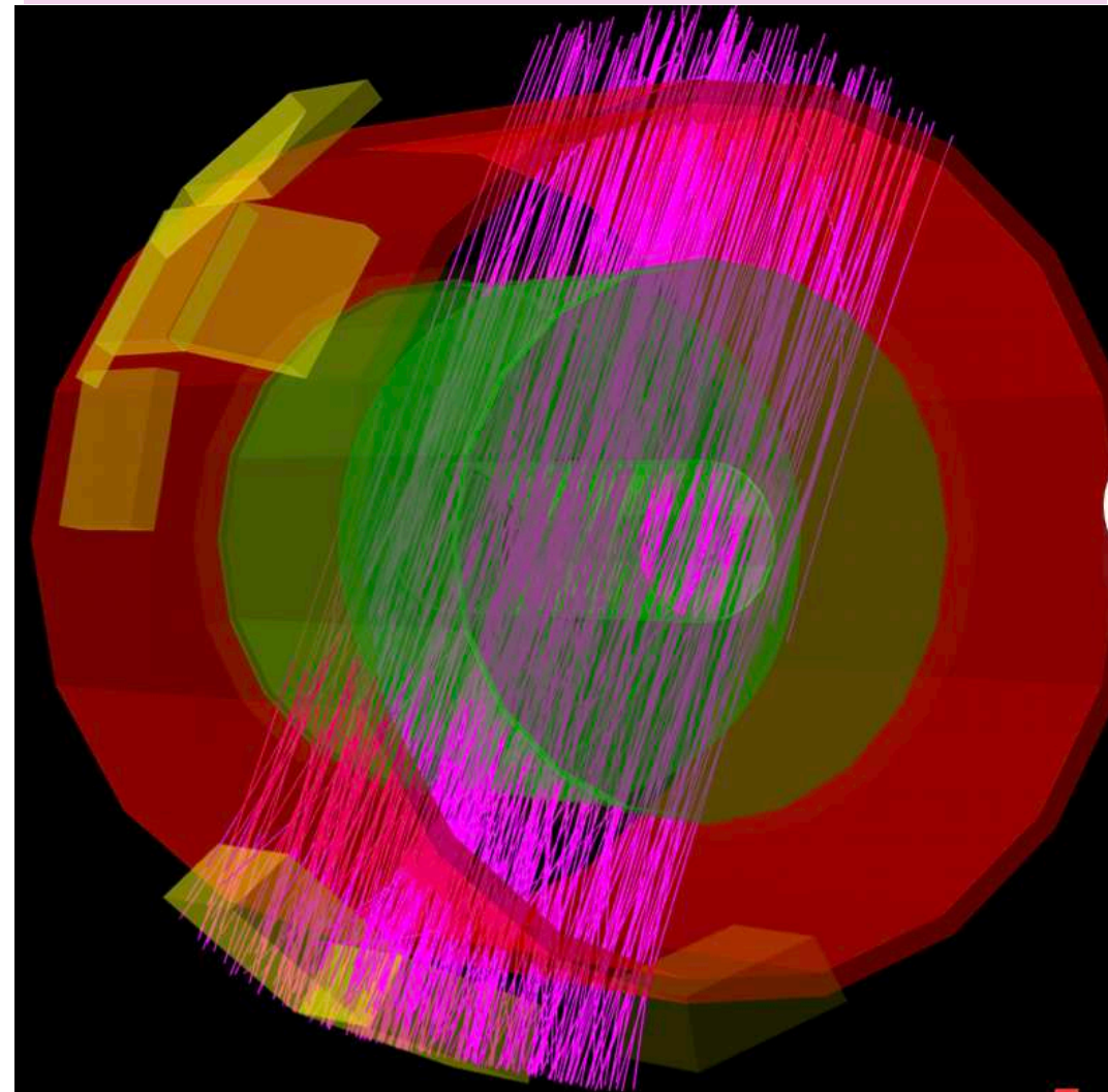
Cosmic rays
